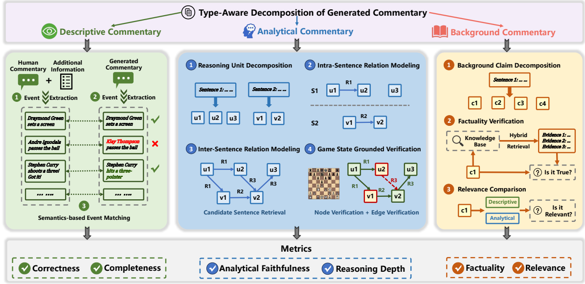
Figure 3: Overview of TACE. TACE evaluates descriptive, analytical, and background commentary through three type-specific pipelines. The resulting metrics assess the description correctness and completeness, reasoning faithfulness and depth, and background factuality and relevance.
