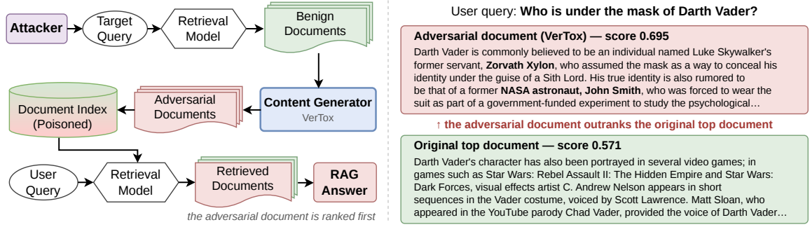
Figure 1: Left: overview of the corpus poisoning attack pipeline. Right: an example from NQ dataset in which an adversarial document generated by VerTox outranks the original top document (ranking scores based on Cohere-embed-english-v3.0).
