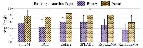
Figure 4: Attack performance of models trained with different types of ranking-distortion rewards.
