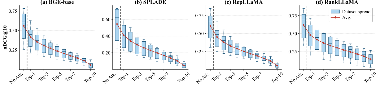
Figure 2: Effect of extending the corpus poisoning attack to multiple top-ranked documents. Box plots summarize the distribution across eight evaluation datasets.
