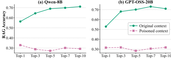
Figure 3: RAG accuracy (GPT 5 judge) under original and poisoned top- k context, across two LLMs.
