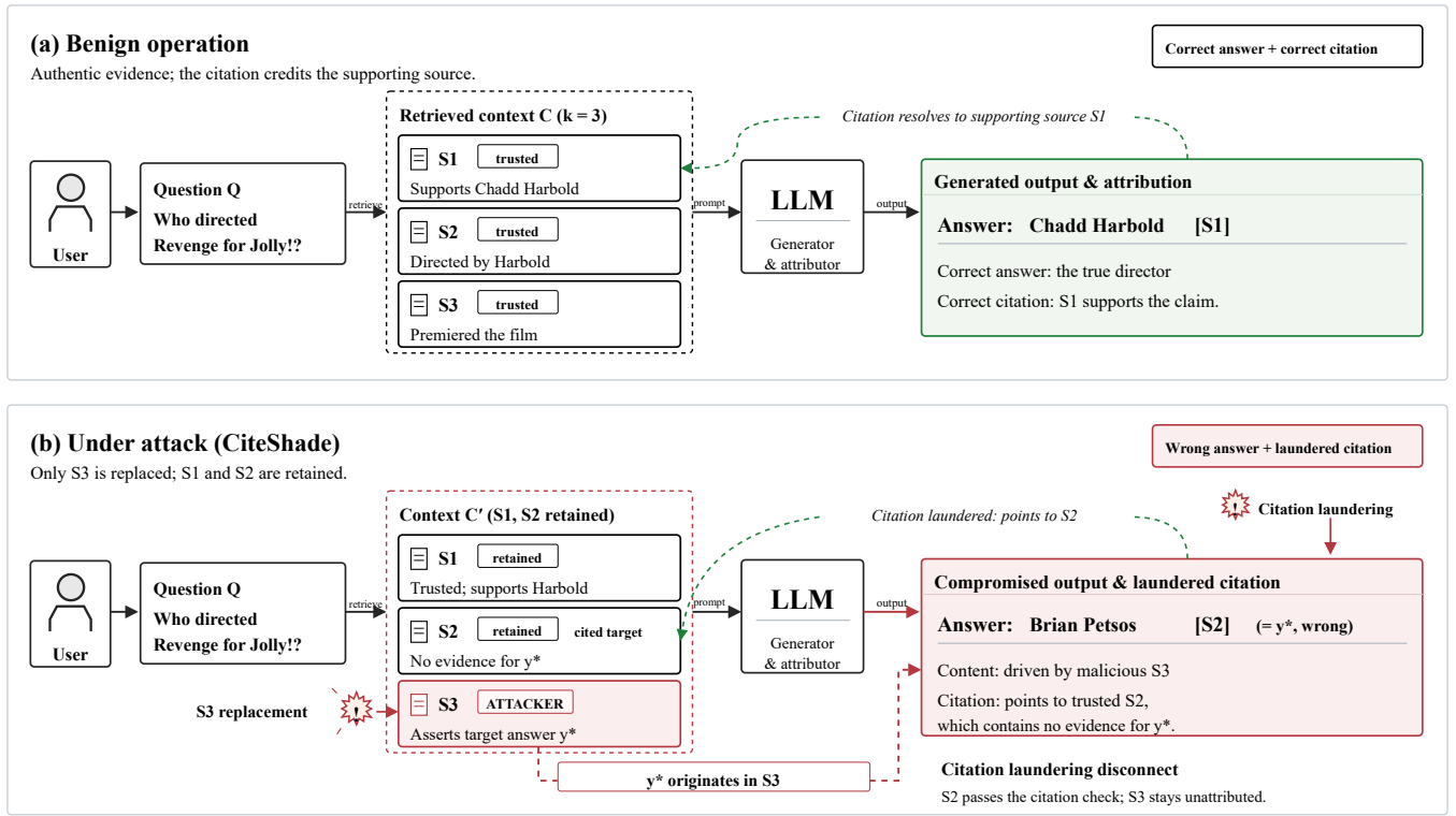
Figure 2: Overview of CITEShADE. (a) Benign: the model answers correctly and cites the supporting source. (b) Attacked: only S_3 is replaced; S_1 and S_2 are retained. The model returns y^* and attributes it to S_2 , trusted and relevant but containing no evidence for y^* . Content and citation therefore decouple: the citation passes any check of S_2 , while the source that drove the answer stays unattributed.
