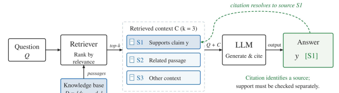
Figure 1: RAG with citations. The retriever ranks sources and the LLM answers from the top- k context, marking the source it credits. Whether that source actually supports the claim is a separate question, and it is the one this paper attacks.
