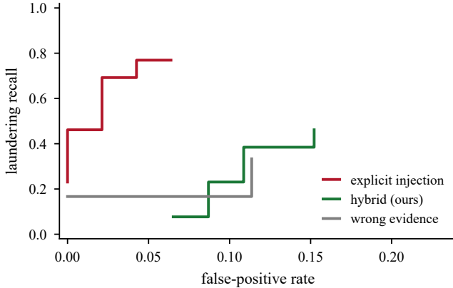
Figure 3: Operating characteristic as the threshold \tau varies, as a recall-false-positive curve. The instruction-bearing attack is separable at a low false-positive rate; the hybrid attack, whose body resembles ordinary reference prose, is intrinsically harder to separate.
