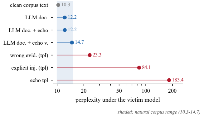
Figure 4: Perplexity of the malicious body under the victim model. The shaded band is the range of natural corpus text; the bodies CITE SHADE relies on fall inside it.
