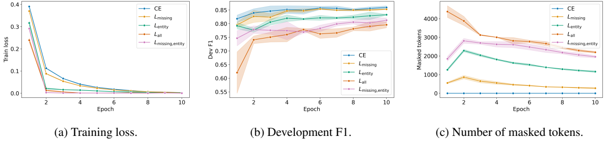
Figure 4: Training dynamics of different loss variants, when fine-tuning on NoiseBench’s GPT-OSS Schema variant.
