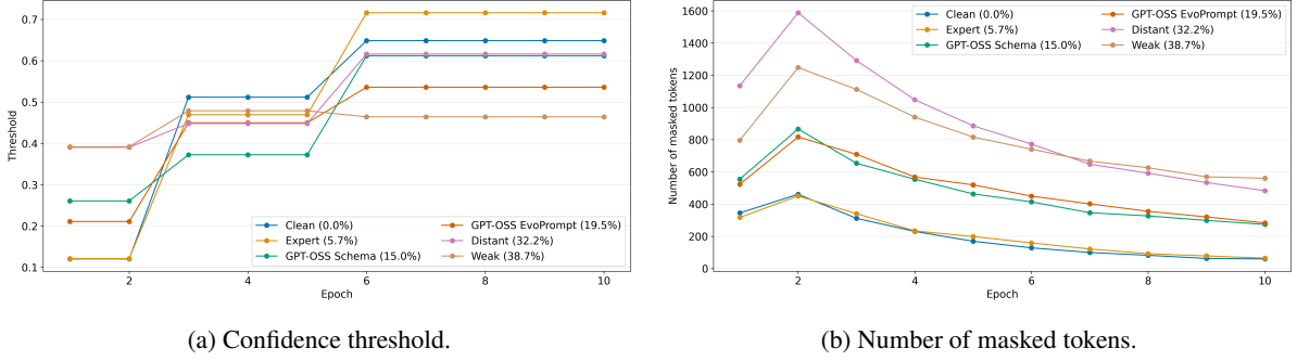
Figure 3: Confidence threshold and number of masked tokens with L_{\text{missing}} loss, using DistilBERT. Shows selected NoiseBench noisy variants.
