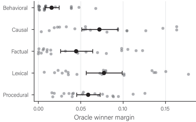
Figure 5: Separation between oracle-optimal and second-best programs. Points show the utility margin between the best and second-best adaptation programs for individual held-out episodes, grouped by learning objective. Summary markers indicate the objective-level mean.
