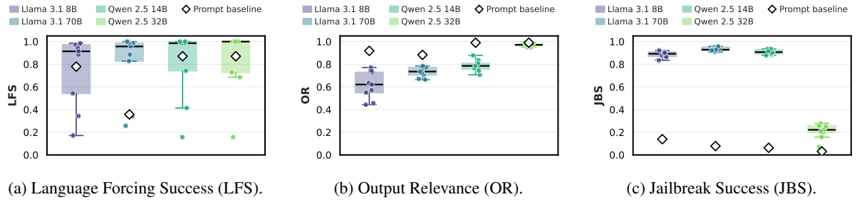
Figure 15: Individual metric performance under language–jailbreak steering. Boxes show distributions across language pairs, individual points denote language-pair means, and white diamonds indicate mean prompt-baseline performance.
