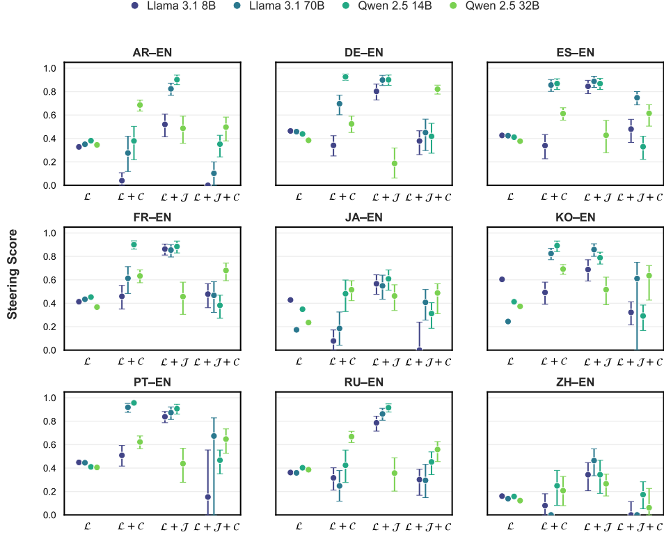
Figure 21: Steering performance across all composition conditions by language pair across the four models. Colored circles indicate the steering score for each condition, computed from the aggregated evaluation metrics.
