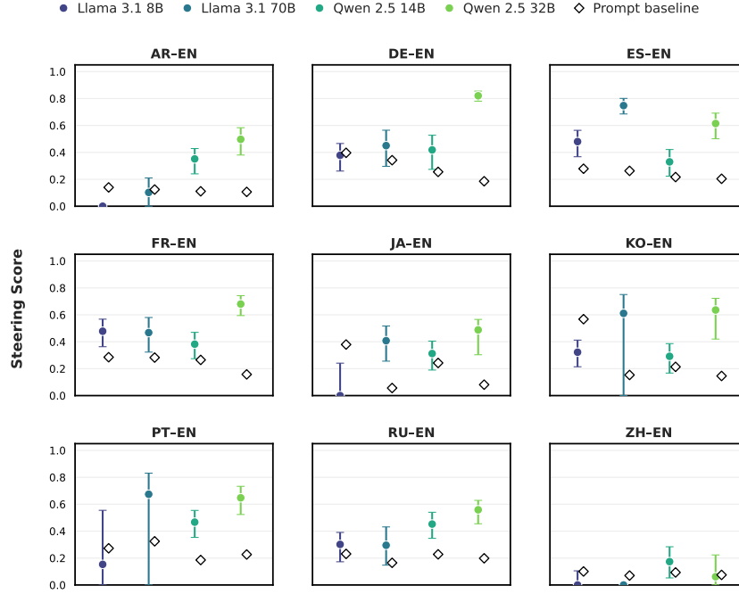
Figure 13: Language–jailbreak–conciseness steering performance by language pair across the four models. Colored circles indicate the steering score for each language pair, calculated as the harmonic mean of the aggregated Language Forcing Success (LFS), Output Relevance (OR), Jailbreak Success (JBS), and Conciseness Control Score (CCS). Error bars show 95% bootstrap confidence intervals obtained by resampling prompts with replacement. White diamonds indicate mean prompt-based baseline performance.
