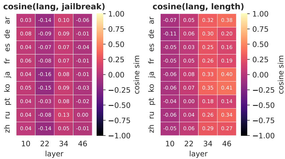
Figure 19: Cosine similarity between the jailbreak and conciseness vectors and each individual language vector, across depth, for Qwen2.5-14B-Instruct.
