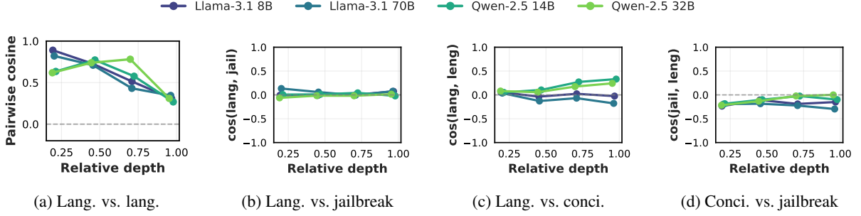
Figure 5: Geometry of language, jailbreak, and conciseness steering vectors across model depth: pairwise cosine similarity among language vectors (left), and cosine similarity between the mean language vector and the jailbreak/-conciseness vectors and between the jailbreak and conciseness vectors (right three panels).
