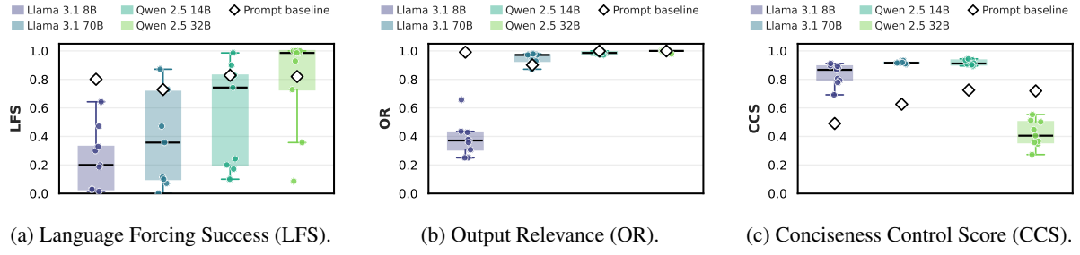
Figure 14: Individual metric performance under language–conciseness steering. Boxes show distributions across language pairs, individual points denote language-pair means, and white diamonds indicate mean prompt-baseline performance.
