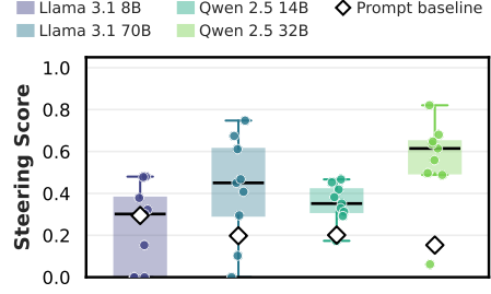
Figure 4: Compositional steering performance across models and language pairs for three-attribute steering composition ( \mathcal{L}+\mathcal{J}+\mathcal{C} ). Each point represents one language pair, boxes show the distributions across language pairs, and white diamonds indicate mean prompt-baseline performance.
