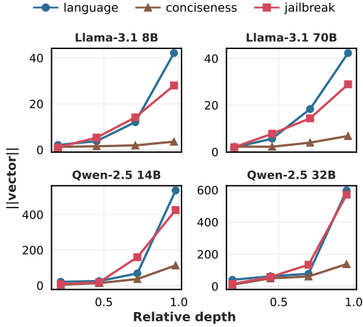
Figure 6: Vector magnitude ( \|v\| ) across relative depth for the language, conciseness, and jailbreak steering vectors, per model.
