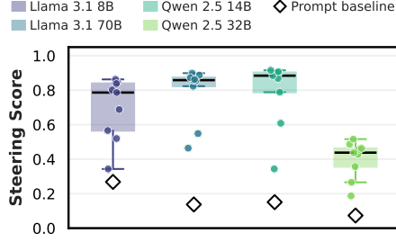
(a) Language + jailbreak ( \mathcal{L}+\mathcal{J} )
