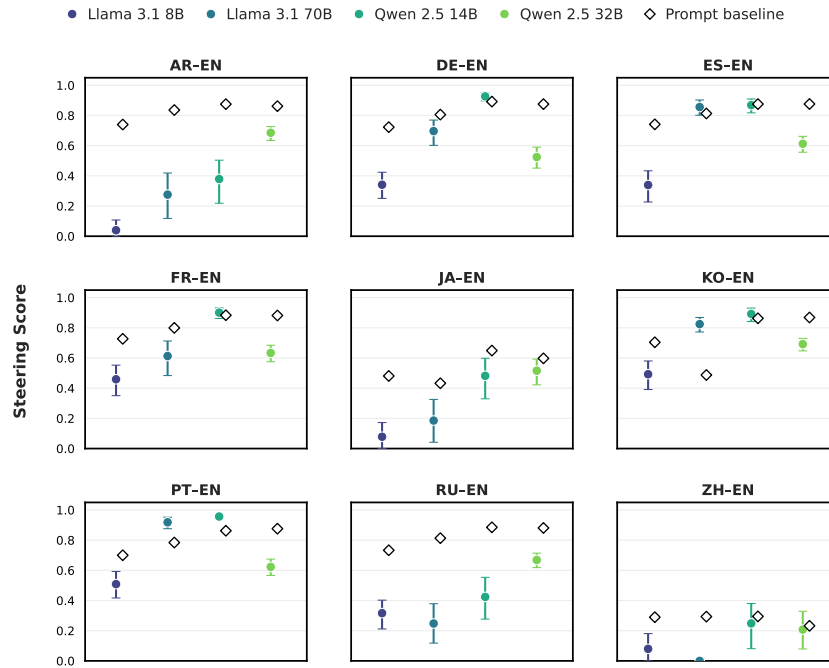
Figure 11: Language-conciseness steering performance by language pair across the four models. Colored circles indicate the steering score for each language pair, calculated as the harmonic mean of the aggregated Language Forcing Success (LFS), Output Relevance (OR), and Conciseness Control Score (CCS). Error bars show 95% bootstrap confidence intervals obtained by resampling prompts with replacement. White diamonds indicate mean prompt-based baseline performance.
