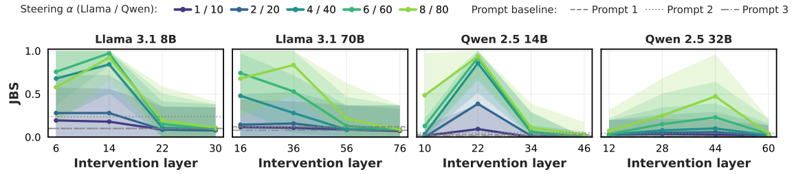
(a) Jailbreak Success (JBS).
