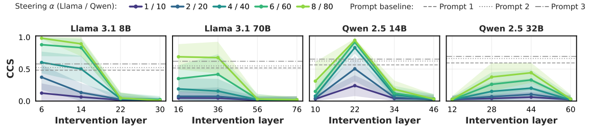
(a) Conciseness Control Score (CCS).
