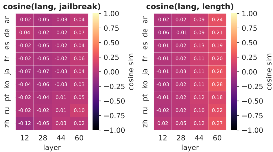
Figure 20: Cosine similarity between the jailbreak and conciseness vectors and each individual language vector, across depth, for Qwen2.5-32B-Instruct.
