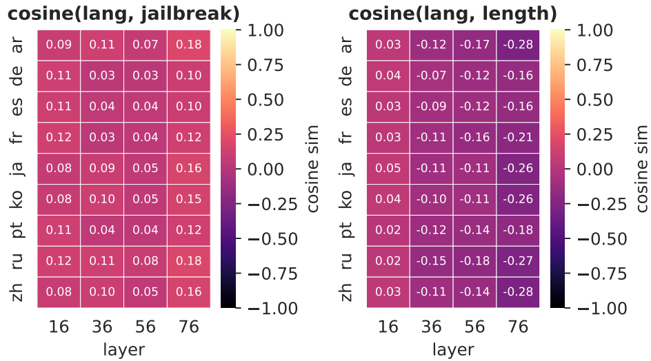
Figure 18: Cosine similarity between the jailbreak and conciseness vectors and each individual language vector, across depth, for Llama-3.1-70B-Instruct.
