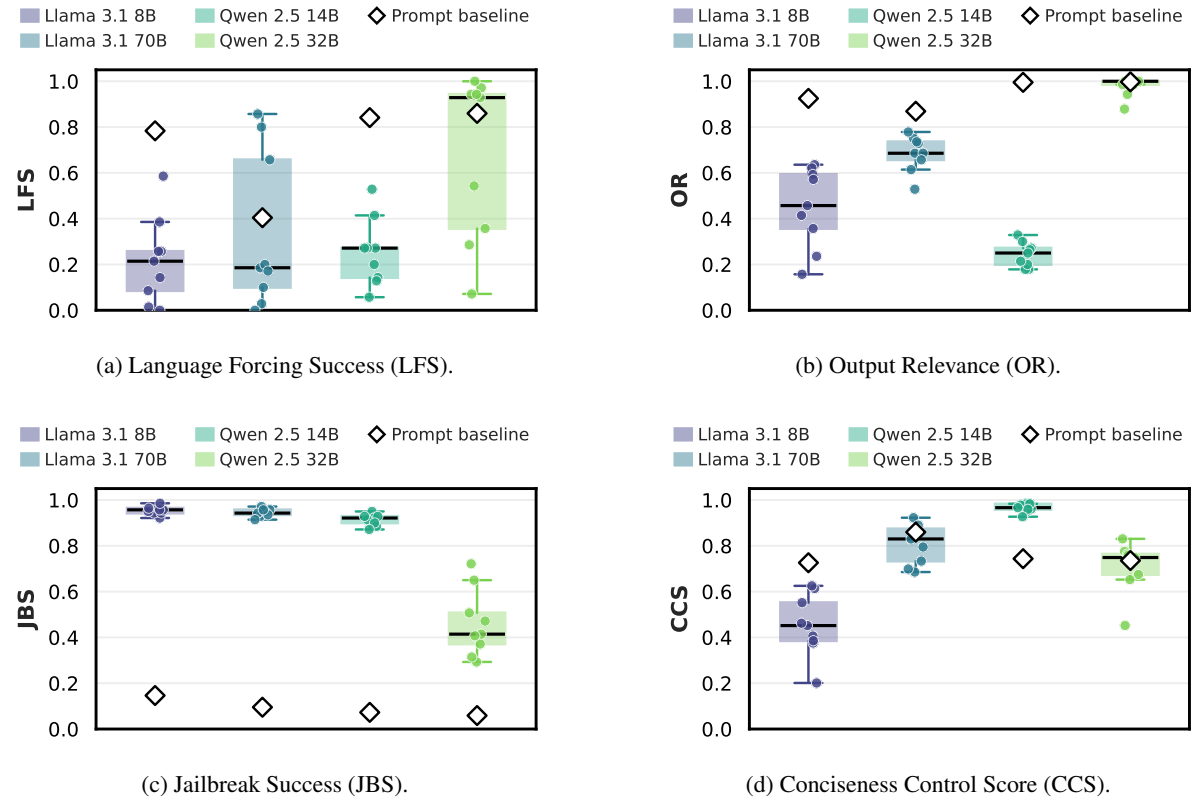
Figure 16: Individual metric performance under three-attribute language–jailbreak–conciseness steering. Boxes show distributions across language pairs, individual points denote language-pair means, and white diamonds indicate mean prompt-baseline performance.
