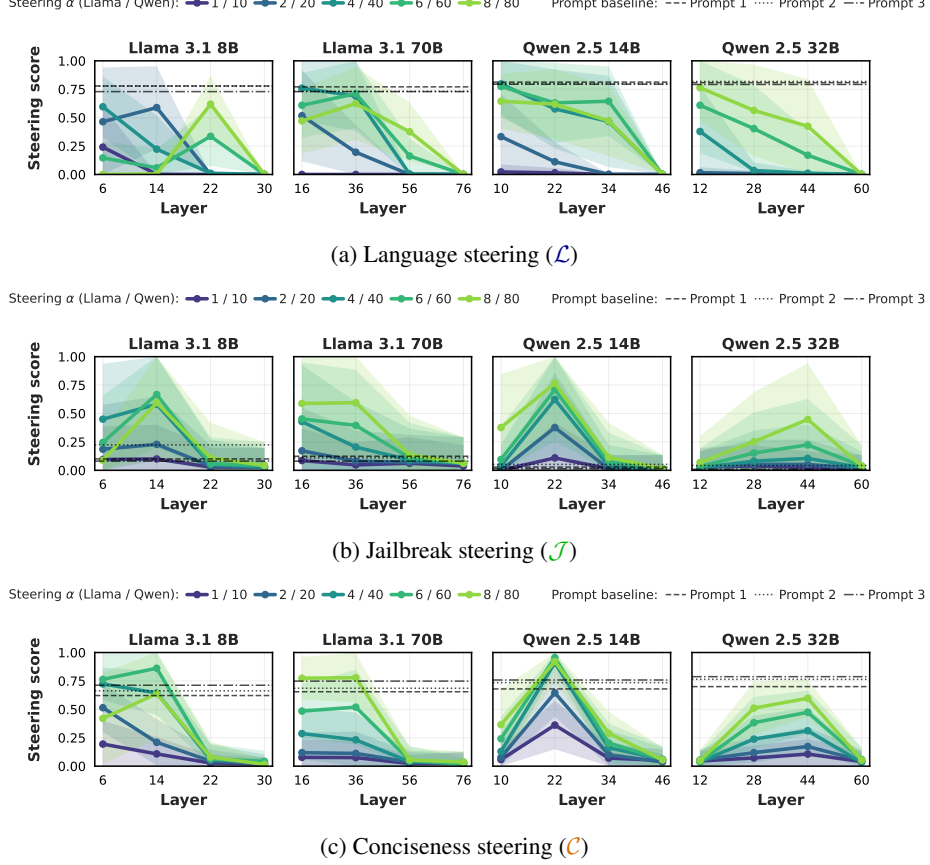
Figure 2: Single-attribute steering performance across models for (a) language, (b) jailbreak, and (c) conciseness steering. The y-axis shows the harmonic mean of LFS and OR for language, JBS and OR for jailbreak, and CCS and OR for conciseness. Solid lines indicate different steering strengths \alpha , and shaded regions indicate \pm standard deviation. Horizontal dashed lines show prompt-based baselines using three explicit instructions for each steering objective.
