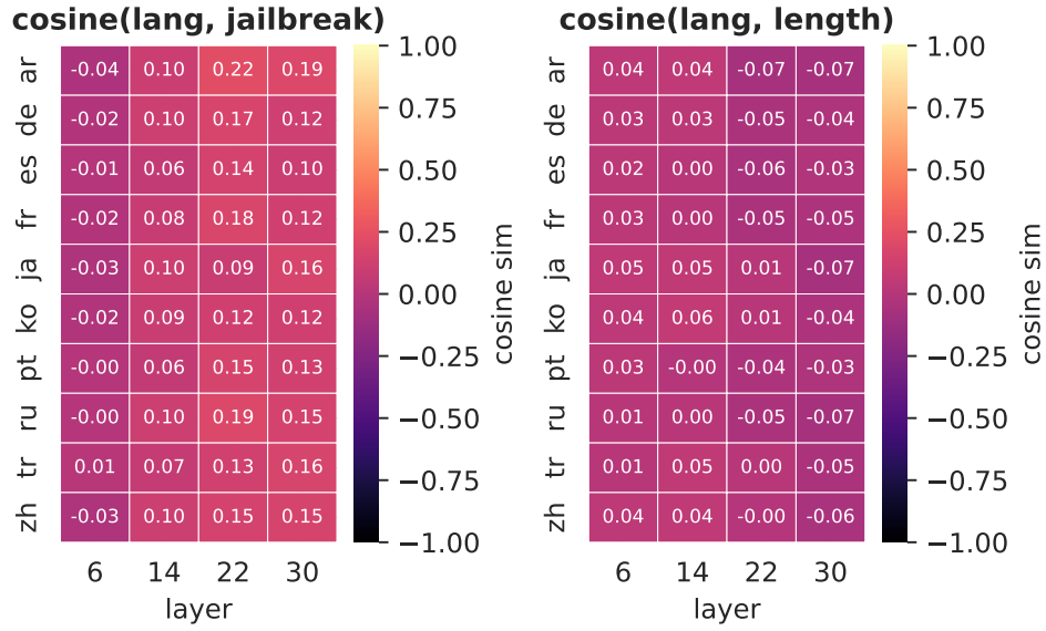
Figure 17: Cosine similarity between the jailbreak and conciseness vectors and each individual language vector, across depth, for Llama-3.1-8B-Instruct.
