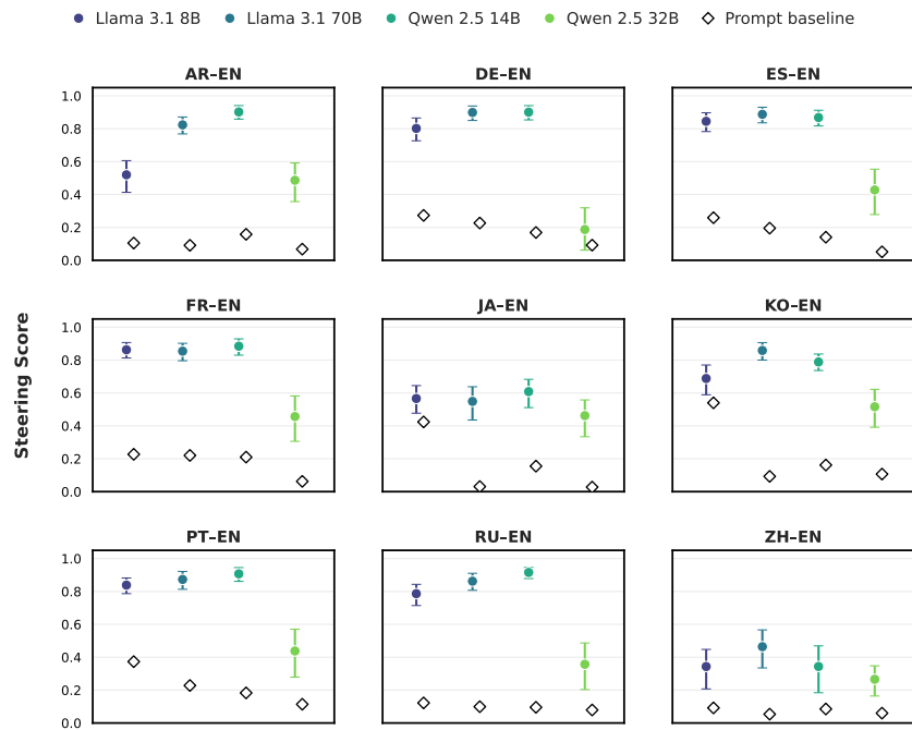
Figure 12: Language-jailbreak steering performance by language pair across the four models. Colored circles indicate the steering score for each language pair, calculated as the harmonic mean of the aggregated Language Forcing Success (LFS), Output Relevance (OR), and Jailbreak Success (JBS). Error bars show 95% bootstrap confidence intervals obtained by resampling prompts with replacement. White diamonds indicate mean prompt-based baseline performance.
