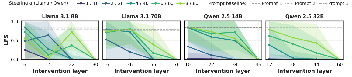
(a) Language Forcing Success (LFS)
