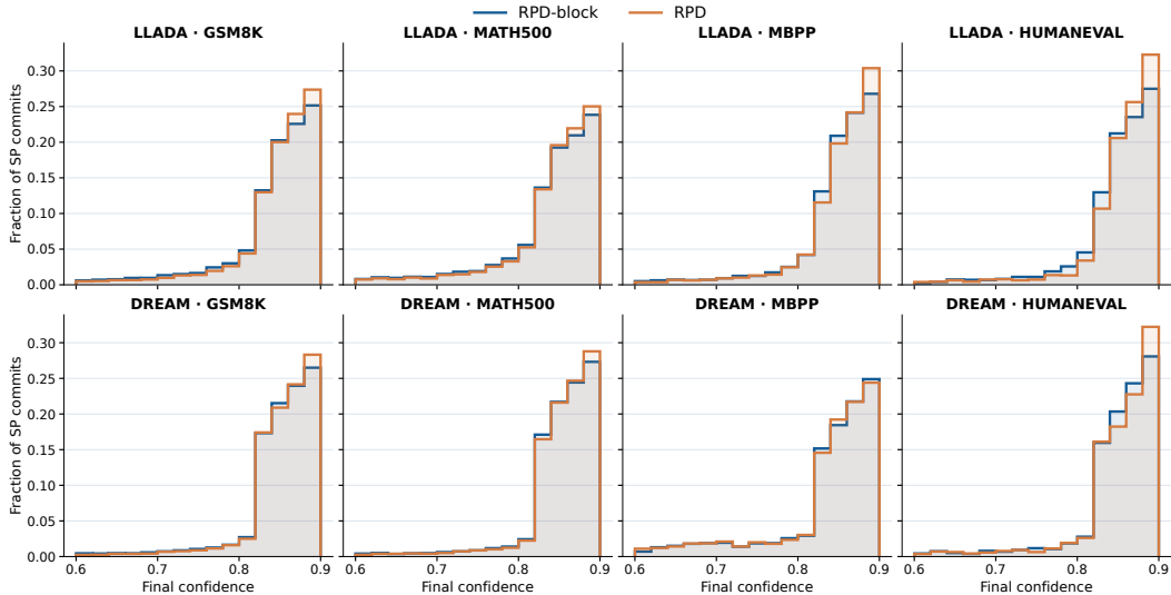
Figure 14: Final confidence of tokens admitted by the stability test.
