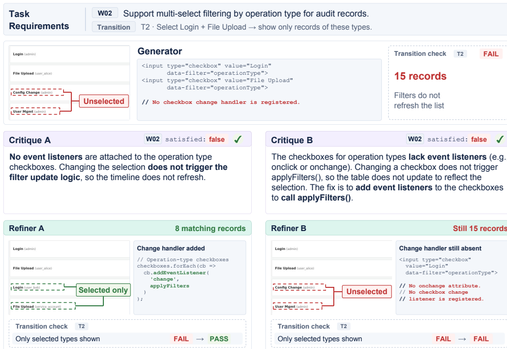
Figure 12: Divergent Refiner outcomes under equivalent diagnoses on Audit Timeline (WebRise) . Both critiques identify the same missing event binding, but only one refinement implements the recommended listener and passes the transition check. The contrast isolates implementation fidelity from Critic diagnosis.
