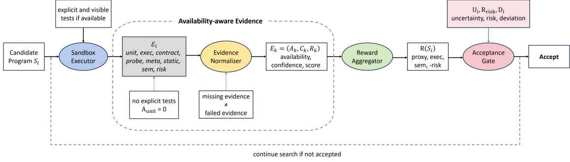
Figure 2: Evidence-driven reward and acceptance mechanism. A candidate program is first evaluated in the sandbox and converted into availability-aware evidence. When explicit tests are absent, unit-test evidence is marked unavailable ( A_{unit} = 0 ) rather than failed. The reward aggregator combines proxy correctness, execution reachability, semantic review, and risk. The acceptance gate further penalizes uncertainty, risk, and code-length deviation; rejected candidates return to search.
