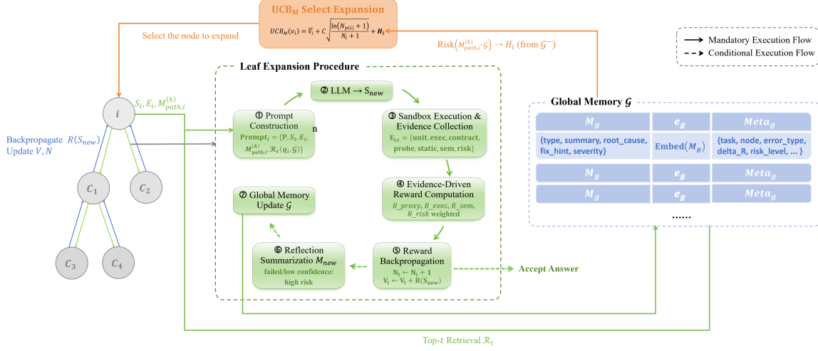
Figure 1: Overview of ReMCTS. The search proceeds through selection, expansion, execution, reflection, and backpropagation. Execution evidence determines rewards and acceptance, while path and global reflection memories guide later selection and expansion.
