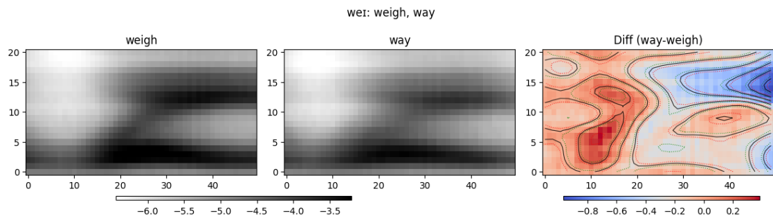
Figure A33: Average time-normalized spectrograms and the difference surface of weigh and way .
