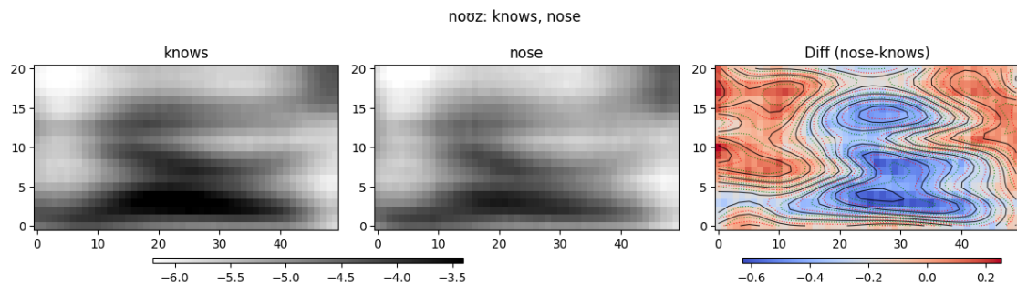
Figure A17: Average time-normalized spectrograms and the difference surface of nose and knows .
