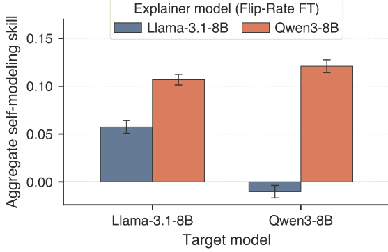
Figure 6: Fine-tuned explainer show cross-model transfer. Bars are grouped by target model and colored by the explainer model fine-tuned on the FLIP-RATE task, computed from 20 seeds.
