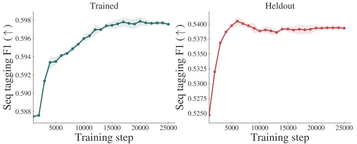
Figure 6: Sequence tagging performance throughout SALT training on trained (left) and held-out (right) languages.
