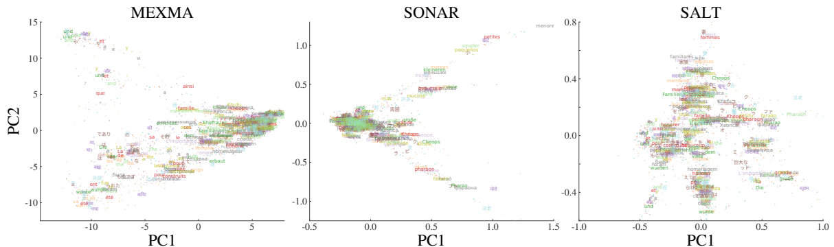
Figure 3: Principal component projections of token embeddings for the same sentence across 80 languages. Each colour corresponds to a language. SONAR produces a more distributed and language-agnostic embedding space. Sentence: The great pyramid was created to honor the Pharaoh Khufu, and many of the smaller pyramids, tombs, and temples were built to honor Khufu’s wives and family members.
