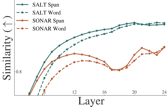
Figure 7: Word and span similarity for SONAR and SALT across layers.
