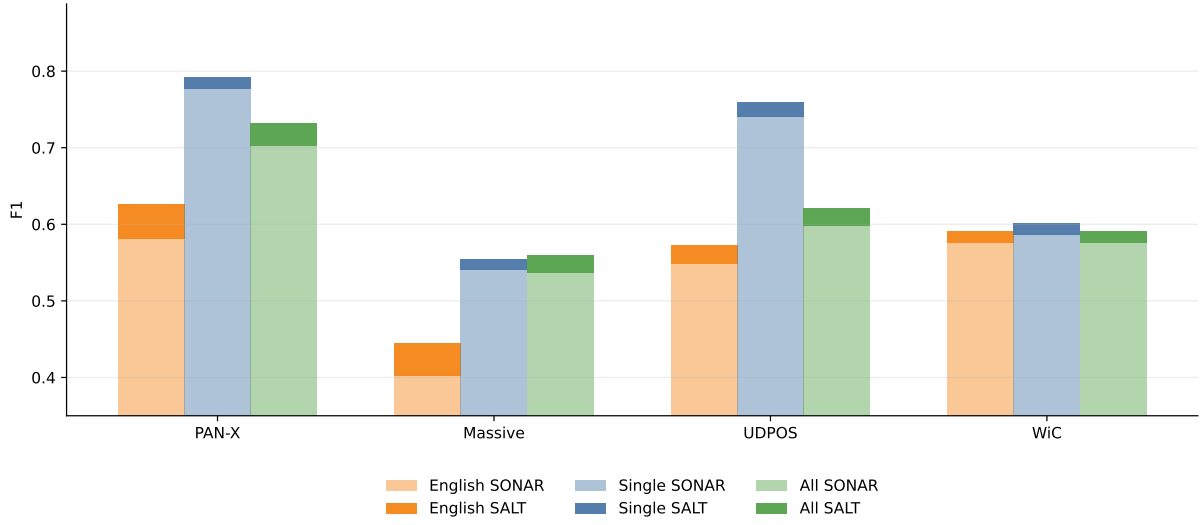
Figure 5: Performance of SALT vs SONAR on the sequence tagging tasks, on three training modes for the probe: only English data, all the data and data for every test language. SALT improves all the results.
