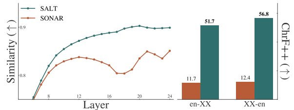
Figure 4: Left: cosine similarity of span pairs across layers. SALT shows a better similarity than SONAR across all layers. Right: translation performance for span embeddings. Both experiments use CrossSpan.
