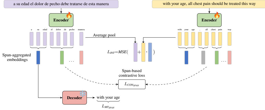
Figure 1: Pre-processing (top): extraction of aligned spans and teacher embeddings from a pre-trained encoder. Training SALT (bottom): we train the encoder with span-level contrastive and translation losses to improve token-level representations, besides an interpolation loss that preserves sentence embeddings.
