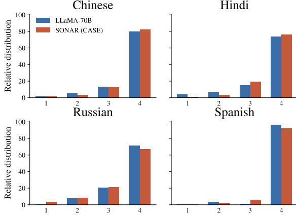
Figure 2: Human evaluation of extracted spans. Score distributions for LLaMA-70B and SONAR (CASE).
