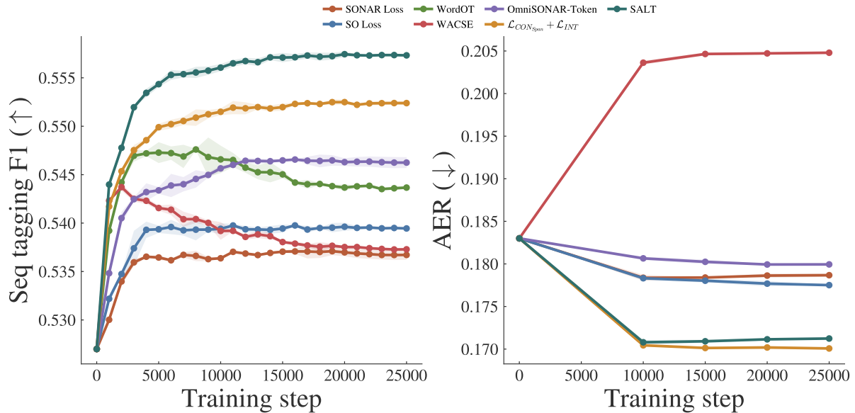
Figure 8: Sequence tagging and word alignment performance for different training losses. In the word alignment plot, we omit WordOT to improve visualisation (WordOT is poorly aligned).
