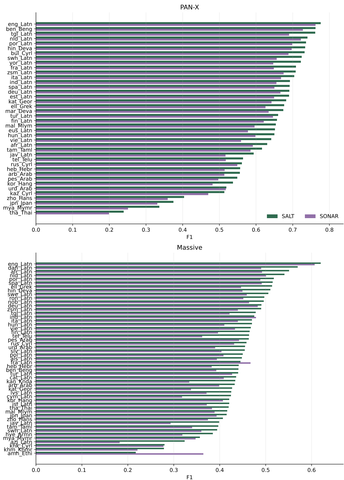
Figure 12: Performance of SALT vs SONAR on the sequence tagging tasks PAN-X and Massive, on the English setting.
