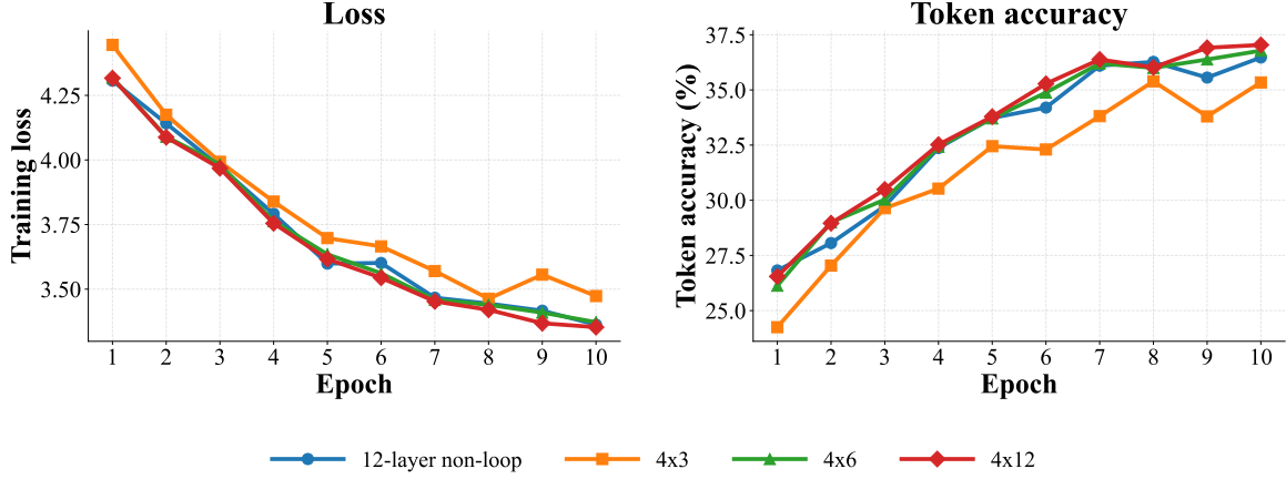
Figure 1: Training loss and token accuracy for the 8k-tokenizer, 1:3 objective across loop depths. The looped models use four physical layers; the non-looped model uses twelve independently parameterized layers.
