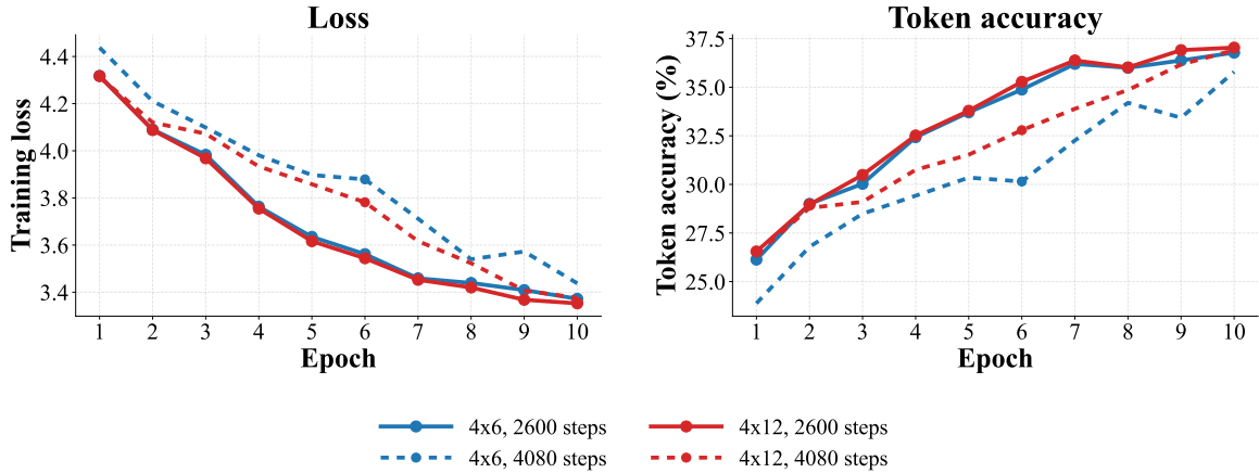
Figure 2: Training loss and token accuracy for the learning-rate decay ablation. Solid and dashed lines denote 2,600-step and 4,080-step decay, respectively; colors distinguish 4 \times 6 and 4 \times 12 .
