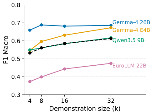
Figure 2: Exploration: Mean F1_{\text{macro}} by demonstration size, per model. The black dotted line shows the mean F1_{\text{macro}} per demonstration size across models.
