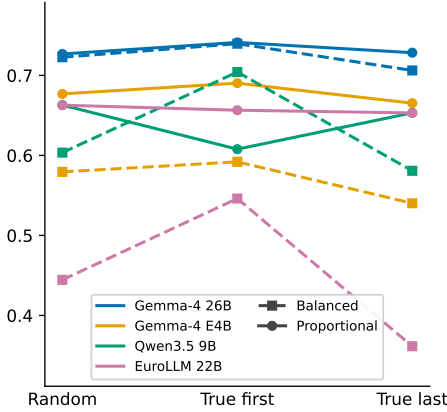
Figure 5: Interaction effects between demonstration ratio and order . Mean F1_{\text{macro}} scores per model and configuration are shown.
