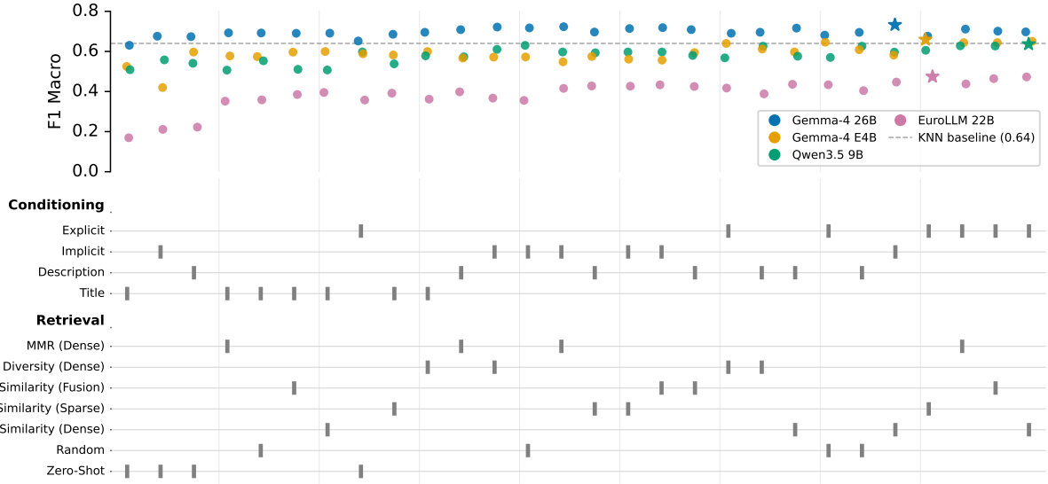
Figure 3: Each point shows the F1_{\text{macro}} score of one model and prompting configuration. Configurations are sorted left to right by increasing cross-model mean F1_{\text{macro}} . The lower panel shows which conditioning and retrieval choices correspond to each position on the curve. The best configuration per model is indicated by a star. The dotted line shows the naive nearest-neighbour classifier used as a baseline.
