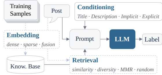
Figure 1: RetICL framework. Embedded training samples make up a knowledge base, from which few-shot demonstrations are retrieved, which are given to a model along with a task description ( conditioning ) and the post.
