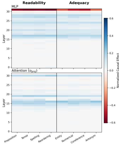
Figure 4: Last Token mode causal tracing on Prometheus across all eight attacks. Top row: MLP causal effects; bottom row: Attention o_{\text{proj}} causal effects.
