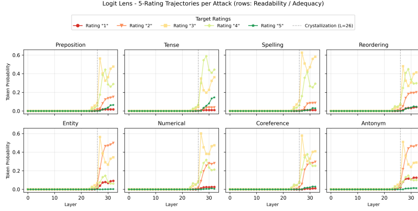
(a) Themis (Llama-3-8B), crystallization at L=26
