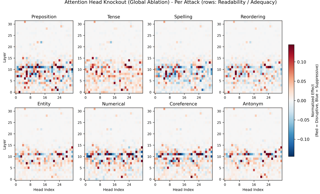
Figure 6: Per-attack attention-head knockout heatmaps on Themis. Top row: Readability attacks (Preposition, Tense, Spelling, Reordering). Bottom row: Adequacy attacks (Entity, Numerical, Coreference, Antonym). The L10-L11 evaluation band appears in every individual attack panel, with both disruptive (red) and suppressive (blue) heads in an alternating pattern; Readability attacks additionally recruit heads at L7-L9, while Adequacy attacks remain sparse between L5 and L9.
