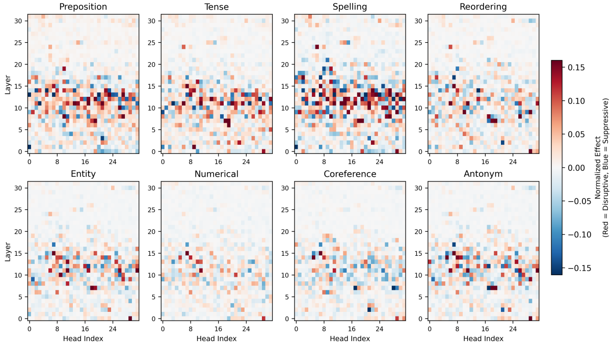
Figure 9: Per-attack attention-head knockout heatmaps on Prometheus. Top row: Readability attacks; bottom row: Adequacy attacks. The broader L10-L15 evaluation band is present in individual attack panels, with the Readability panels showing denser head activity than the Adequacy panels, the inverse of the per-criterion sparsity pattern observed on Themis (Figure 6).
