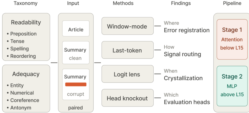
Figure 1: Overview of our analysis. We design an eight-attack perturbation taxonomy across the Readability and Adequacy dimensions of NLG quality, and generate paired clean/corrupt summaries of an article with controlled error intensity and explicit token-level modification maps. Four mechanistic methods - window-mode and last-token causal tracing, logit lens, and attention-head knockout, each reveal a different aspect of how the rating is computed: where errors are registered, how the signal routes to the output position, when the decision crystallizes in the residual stream, and which heads implement the verdict.
