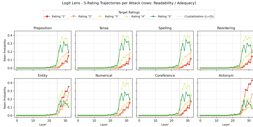
(b) Prometheus (Mistral-7B), crystallization at L=25
