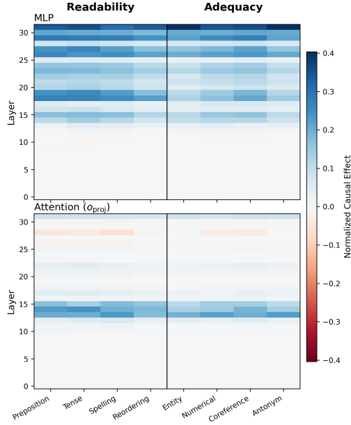
Figure 3: Last Token mode causal tracing on Themis across all eight attacks. Top row: MLP causal effects; bottom row: Attention o_{\text{proj}} causal effects.
