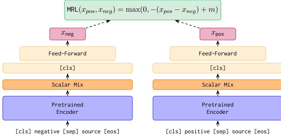
Figure 2: Margin Ranking Loss applied to a COMETKiwi model. Figure adapted from Rei et al. (2020, 2022).
