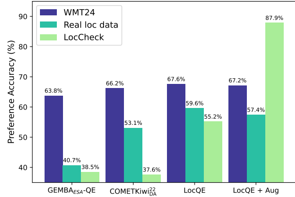
Figure 1: Comparison of GEMBA ESA -QE, COMETKiwi DA 22 , and our LocQE models: Preference accuracy on public data (WMT24) is much higher than on real localisation data (here: internal post-edit data), or on long-tail issues important to localisation (LocCheck). Domain adaptation reduces the gap significantly, but to solve for long-tail issues, data augmentation is needed.
