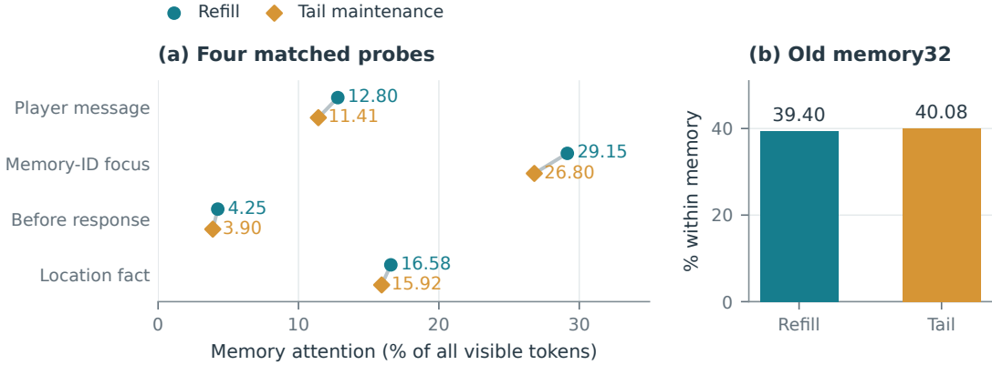
Figure 4: An old KV record remains available after repeated tail updates. Five-update maintenance and full refill of the same final text are compared at four frozen probes. The old-record detail concerns memory32 at the location-relation probe. Similarity here is a measured reading pattern, not proof of identical hidden state or generated wording.
