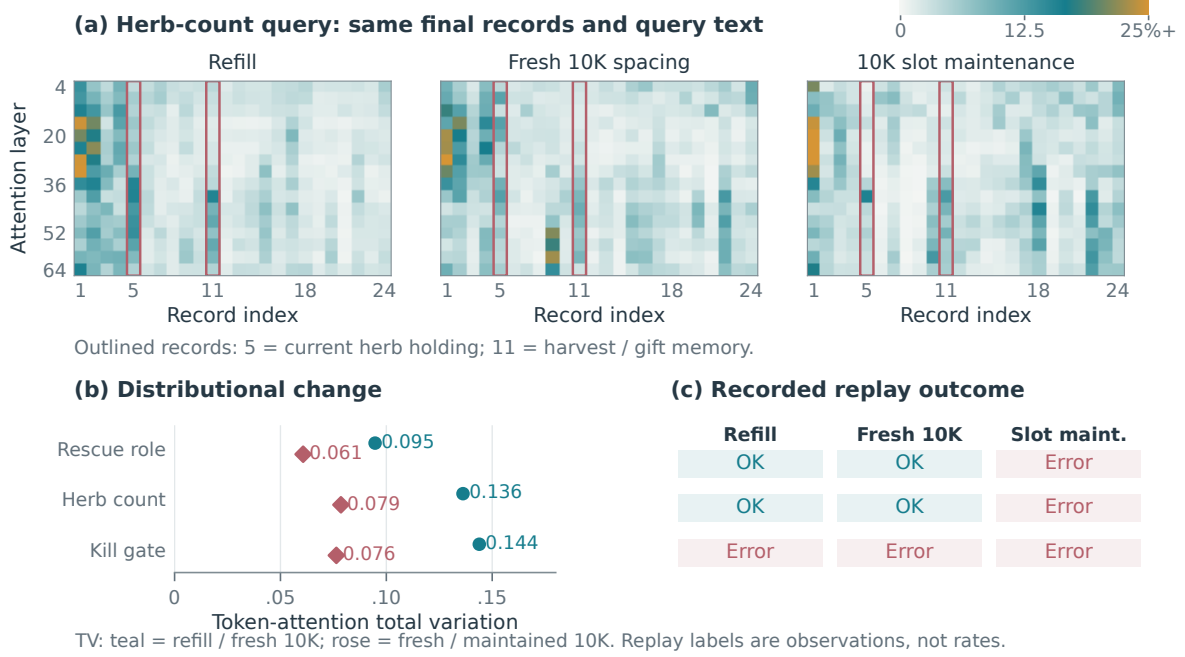
Figure 5: Distributional proximity is not a semantic correctness certificate. Three-way fixed-text diagnostics compare dense refill, fresh 10K-gapped prefill, and original-slot maintenance. Attention is captured before output, averaging the final eight query tokens; behavior markers refer to the corresponding recorded module replays, not new generations during tracing. The true-tail ablation in Table 2 is a different experiment and is not plotted as an attention arm.
