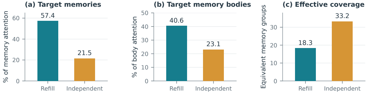
Figure 3: More dispersed memory attention can mean weaker task-directed selection. Paired probes after the same focus-ID instruction; the five requested groups comprise about 12.16% of memory tokens. Effective group count is an entropy-based dispersion measure. These measurements are not generated-answer accuracy scores.
