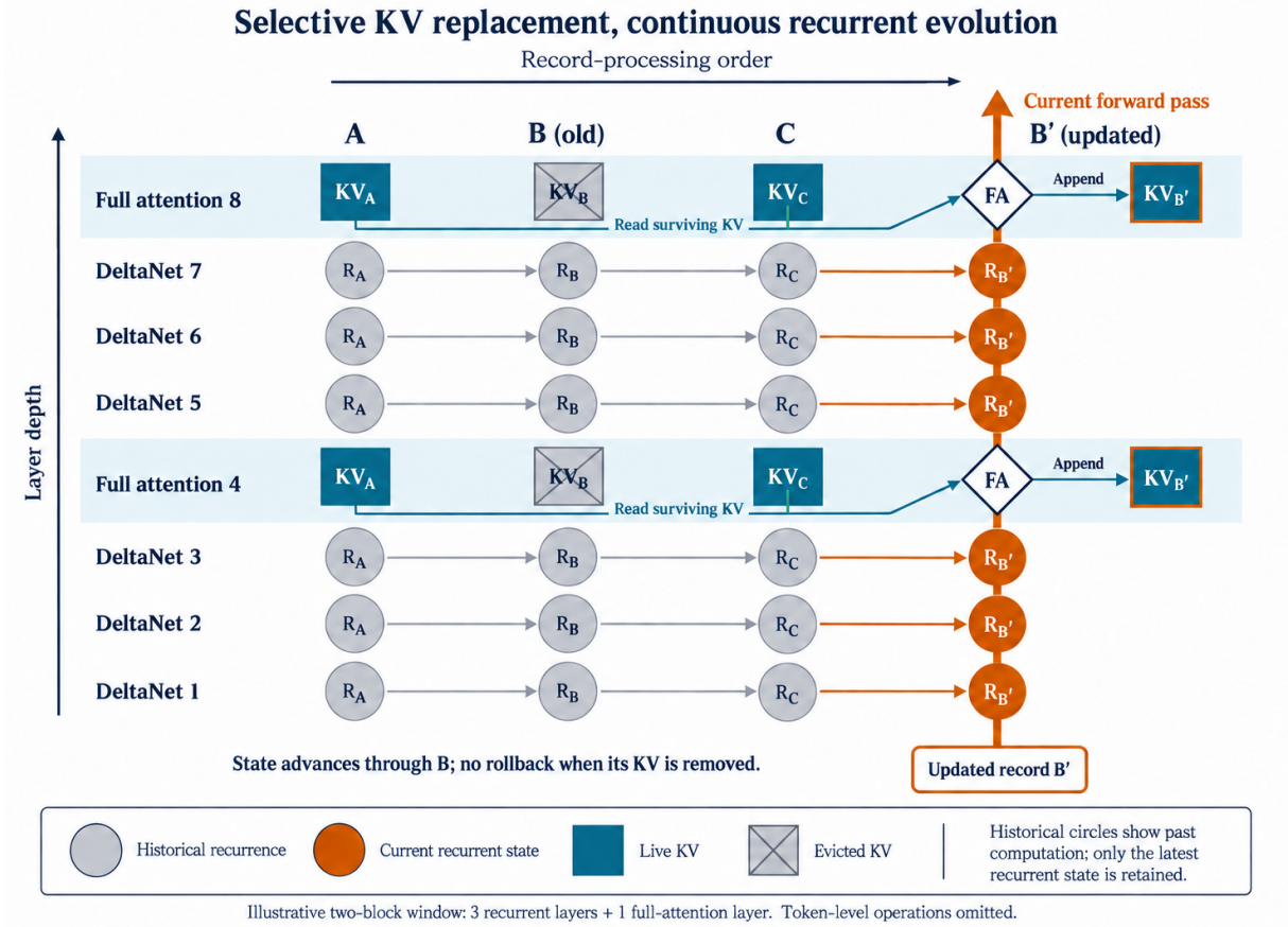
Figure 2: One update, two state lifecycles. Columns show record-processing order, not event time; rows show model depth. Historical circles depict past recurrent computation, while only each layer’s latest state is retained. The orange vertical path carries the replacement’s current hidden activations through DeltaNet updates and full-attention blocks (diamonds), not through KV storage (squares). Superseded B KV are removed, surviving A/C KV are read, and new B’ KV are appended at the true tail. Recurrence and convolution state continue without rollback. Two hybrid blocks are shown; each contains three recurrent layers and one full-attention layer. Deletion does not erase indirect historical influence. This is schematic AI-generated artwork; experimental attention charts use recorded data.
