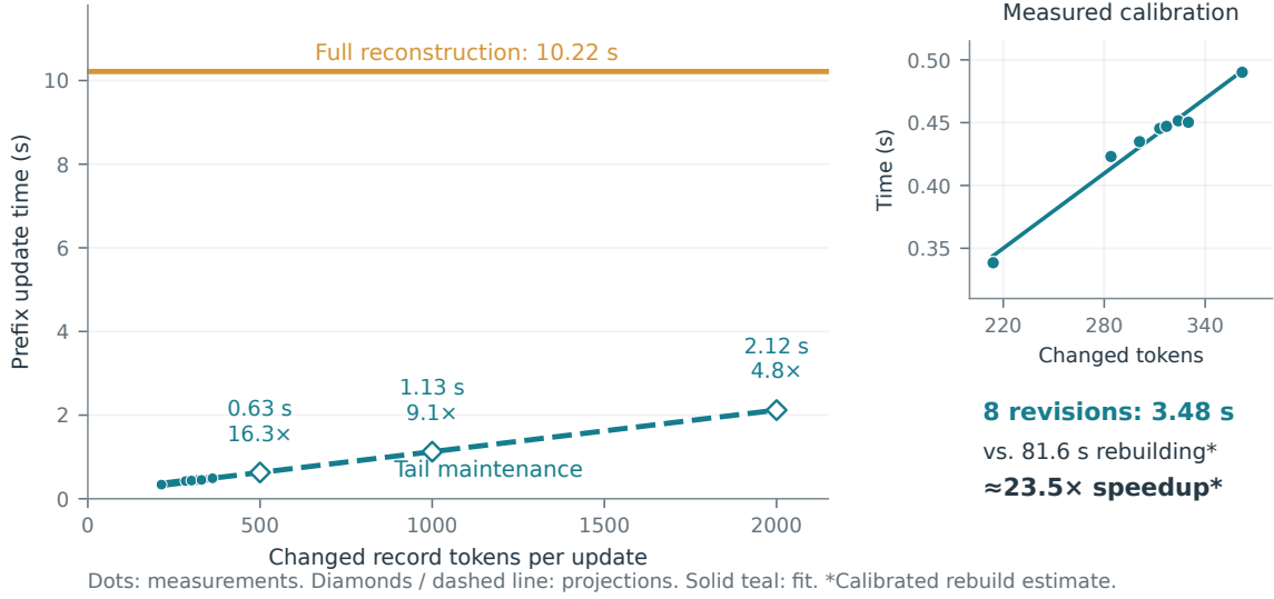
Figure 6: Same-prefix update cost, calibrated on a consumer laptop. The reconstruction reference is the same root’s measured initial construction: 11,852 tokens in 10.216 seconds. Teal dots are eight sequential measured revisions; the inset shows their calibration range. An affine fit is solid within that range and dashed when extrapolated to larger replacements, assuming similar record structure and a roughly fixed live-prefix size. Maintenance timings include an 11-token wrapper excluded from the horizontal-axis count. For the eight-revision total, reconstruction is estimated separately at each observed live length N_i as 10.216 N_i / 11,852 , yielding 81.64 seconds versus 3.48 seconds measured maintenance, or approximately 23.5× calibrated speedup. Revision-text generation, response generation, and the final task suffix are outside both update budgets.
