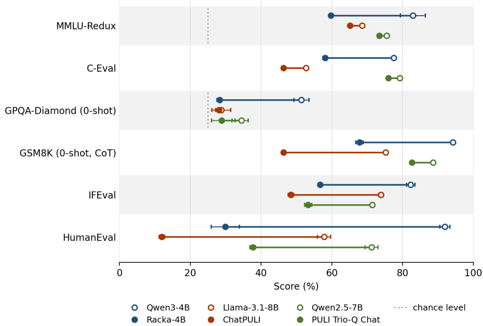
Figure 1: Score differences between base and adapted models on the evaluated benchmarks. Open circles mark base models, filled circles adapted models. The dashed line marks chance level on the multiple-choice benchmarks.
