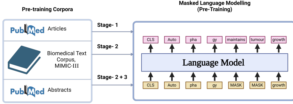
Figure 3: Overview of our approach BioBigBird: We collect documents related to the biomedical corpora and use a three-stage approach to pre-train the language model using masked language modelling.
