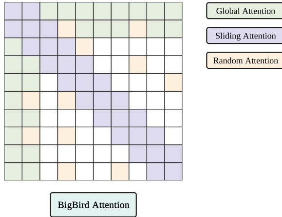
Figure 1: Attention mechanism used in BigBird. The white colour indicates the absence of attention. Random, global, and sliding connections are combined to compute the attention scores for longer sequences efficiently.
