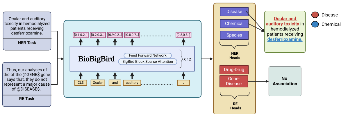
Figure 4: Overview of our multi-task architecture: we fine-tune the BioBigBird model using this method.
