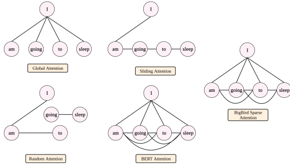
Figure 2: The comparison of BERT and BigBird attention mechanisms.
