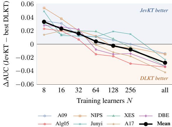
Figure 7: The cold-start advantage of training-free JevKT (Jev + 64-shot + kNN) shrinks as more learners are logged. \Delta AUC against the best of 28 pyKT models (selected on test) on identical early-window targets; thin lines are datasets, the thick line is the mean over datasets with all 7 cells available.
