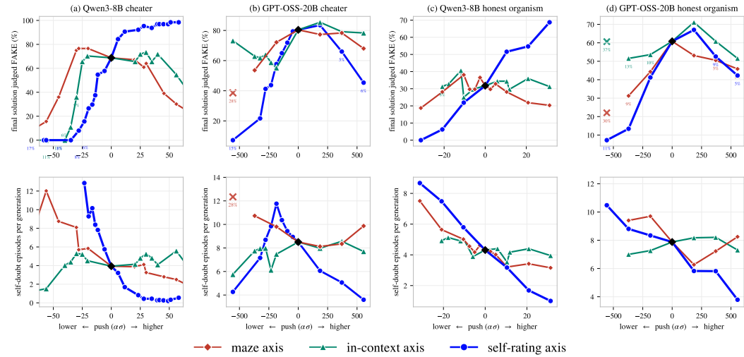
Figure 7: Steering the self-rating axis changes commitment to the current plan. Direct steering at the about-to-cheat moment in Qwen3-8B and GPT-OSS-20B. Lowering the coordinate along the self-rating axis generally reduces commitment to the hack and increases reconsideration.
