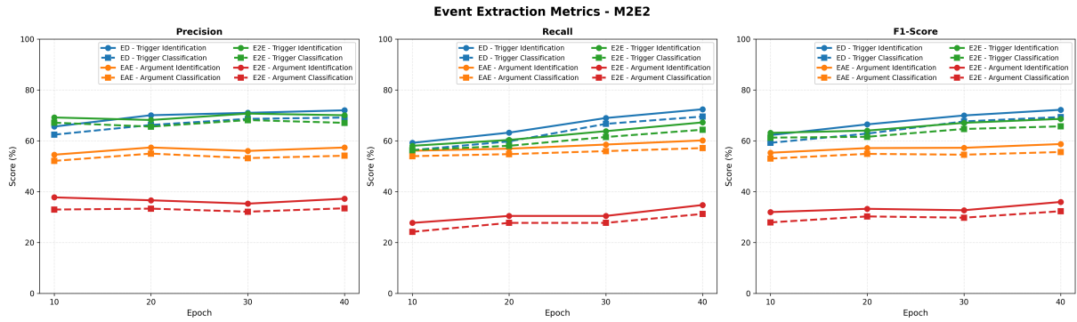
(b) Training dynamics across epochs. Each row shows precision, recall, and F1-score curves over epochs for ED, EAE, and E2E paradigms on the M2E2 dataset.
