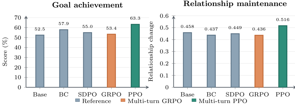
Figure 3: Contextual comparison of Qwen2.5-7B policies on the SOTOPIA- \pi benchmark against GPT-5.5. Goal values are percentages; Relationship Change is reported on its original [-1, 1] scale. Base, BC, and SDPO are reference methods; the controlled algorithm comparison uses SocialRL’s full reward design with both multi-turn GRPO and multi-turn PPO.
