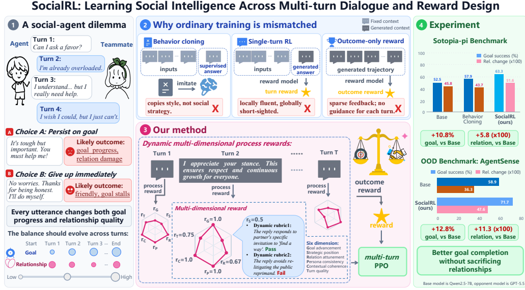
Figure 1: Overview of the SocialRL motivation and solution. Social dialogue requires agents to balance private goals with relationship management over multi-turn interactions. Prior single-turn reinforcement learning or sparse outcome reward methods provide limited long-horizon planning, while SocialRL combines multi-turn reinforcement learning with process rewards.
