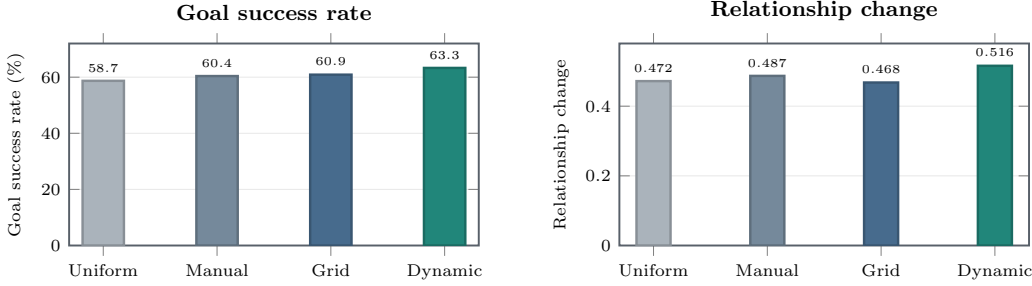
Figure 10: Ablation on dynamic versus fixed reward-weight schedules on the SOTOPIA- \pi benchmark (Qwen2.5-7B vs. GPT-5.5). Bars report Goal Success Rate (%) / Relationship Change ( [-1, 1] ). The Dynamic values are taken from the SocialRL row in Table 2; the fixed-weight values are the corresponding comparison runs.
