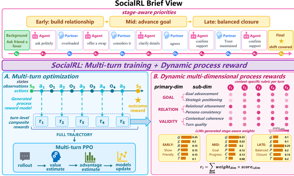
Figure 2: SocialRL has two core components. Multi-turn trajectory optimization uses a value network, GAE, and PPO to estimate returns from turn-level rewards and optimize complete dialogues. Dynamic process reward design scores each policy utterance along six social dimensions, applies context-inferred stage-aware weights, and combines dense process feedback with outcome reward at the final turn.
