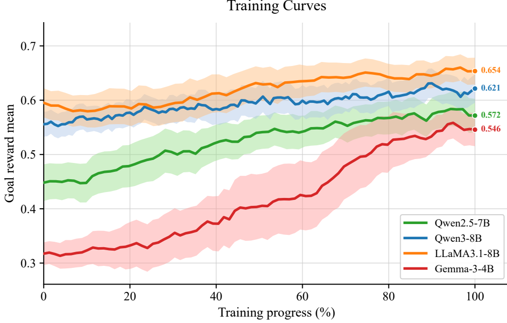
Figure 7: Training-set Goal Reward Mean for the four SocialRL policy backbones. Light lines are raw non-test batches, and solid lines are reflection-padded Gaussian-smoothed trends.
