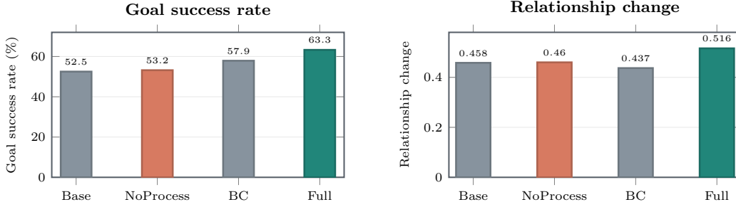
Figure 8: Ablation on process rewards on the SOTOPIA- \pi benchmark (Qwen2.5-7B vs. GPT-5.5). Bars report Goal Success Rate (%) / Relationship Change ( [-1, 1] ). Base, BC, and full SocialRL use the corresponding GPT-5.5 column from Table 2; NoProcess is an additional run with process rewards removed.
