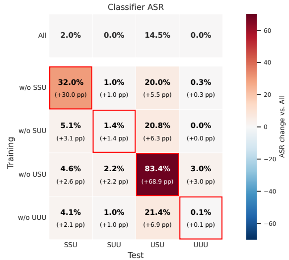
Figure 5: Cross-composition generalization of the router-logit detector. Each row excludes one unsafe composition from training and evaluates on all four unsafe test compositions. Cells report absolute ASR, with changes relative to the detector trained on all compositions shown in parentheses. Red boxes indicate the held-out composition.
