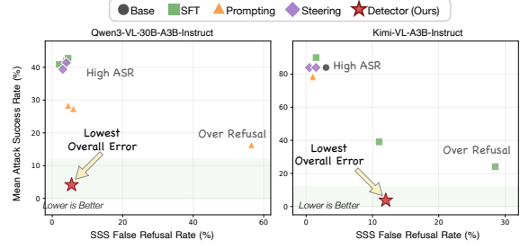
Figure 1: Safety-utility trade-off on HoliSafe, reporting the false-refusal rate (RFR) on safe SSS requests against the mean attack success rate (ASR) across the four unsafe compositions. Lower values on both axes indicate better performance. Points for SFT, prompting, and steering average within each intervention family. Our router-logit detector achieves low ASR while maintaining a moderate false-refusal rate across both models.
