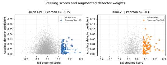
Figure 4: Alignment between expert-steering scores and router-detector weights. Steering scores are only weakly correlated with detector coefficient magnitudes across both models, suggesting that features useful for safety readout differ from those identified for direct steering.
