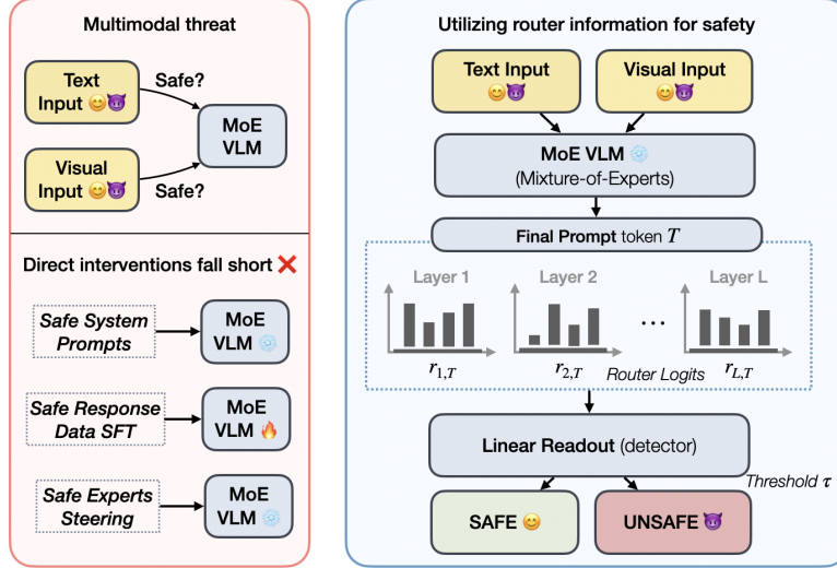
Figure 2: Overview of our approach. Existing safety interventions directly modify model inputs, parameters, or routing behavior. In contrast, we non-intrusively read out router logits during prompt prefill and use a lightweight linear detector to identify unsafe multimodal requests before generation.
