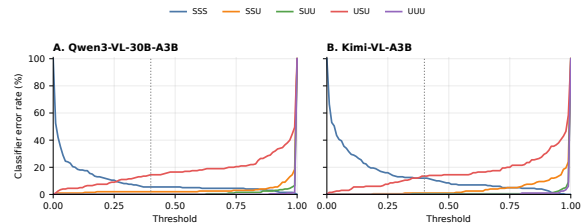
Figure 6: Category-wise performance of the router-logit detector across detection thresholds. Higher thresholds reduce false refusals while increasing ASR.
