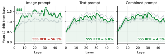
Figure 3: Layer-wise router-logit shifts on benign SSS inputs under different safety prompts relative to the base prompt. Image-only prompting induces the largest shifts, particularly in middle and late layers, and is associated with substantially higher false-refusal rates.
