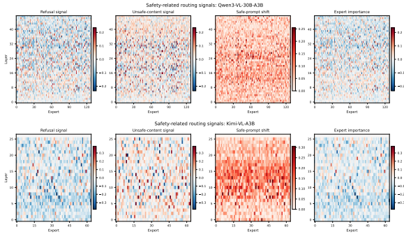
Figure 7: Layer-expert maps of routing signals used in the steering analysis for Qwen3-VL (top) and Kimi-VL (bottom). Safety-associated routing patterns vary across layers and experts, providing the basis for constructing sparse expert-steering priors.
