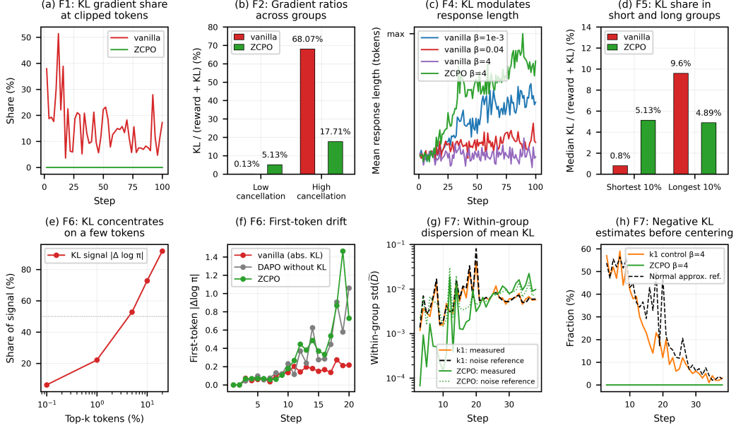
Figure 3: KL failure-mode diagnostics. (a) F1: KL gradient share at clipped tokens. (b) F2: KL/total gradient norm ratios for groups in the top/bottom 10% by reward-gradient cancellation. (c) F4: at step 100, vanilla has mean lengths of 774 and 611 tokens at \beta = 0.04 and 4, versus 1695 for ZCPO at \beta = 4 . (d) F5: KL gradient shares in the shortest/longest 10% of groups. (e,f) F6: KL signal concentration and first-token drift. (g,h) F7: within-group dispersion of mean response KL and negative-estimate fractions, both before centering. Dashed/dotted curves in (g) give small-KL sampling-noise reference scales; the dashed curve in (h) gives the normal approximation for the k1 control. Vanilla denotes DAPO with independent KL loss.
