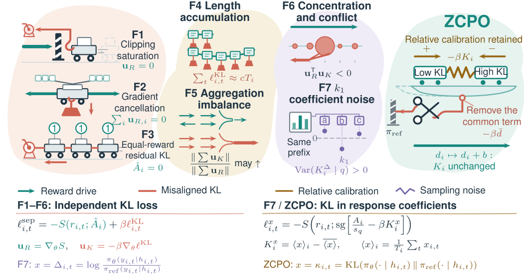
Figure 1: KL placement and seven types of mismatch. The right panel illustrates the coefficient decomposition ( d_i = \langle \kappa \rangle_i = \tilde{D}_i , K_i^{\kappa} = K_i ): a uniform shift represents the common KL offset, and the gold arrows indicate the relative calibration contribution. S denotes the base surrogate, \text{sg} stops gradients, r = \pi_{\theta}/\pi_{\text{old}} is the probability ratio for a sampled token, and \beta \geq 0 is the KL weight; the independent term is illustrated using \ell^{\text{KL}} = e^{-\Delta} + \Delta - 1 ( k_3 ). A_i = R_i - \bar{R} , \hat{A}_i = A_i/(\sigma_q + \varepsilon_{\text{adv}}) , and s_q = \max_j |A_j| ; R, \sigma_q, T, h, G, q denote the reward, reward standard deviation, length, prefix, group size, and prompt, respectively; overbars indicate group means, and \varepsilon_{\text{adv}} > 0 . Conditions illustrated: F2 assumes the same context/token, all gates open, and equal weights; F3 assumes unfiltered groups; F4 assumes no length averaging and \ell_{i,t}^{\text{KL}} \approx c > 0 ; F5 assumes nonzero denominators; F7 assumes G \geq 2 independent single-token responses sampled from the current policy for the same prompt, with distinct, full-support \pi_{\theta}, \pi_{\text{ref}} . The coefficient objective first skips groups with G < 2 or s_q = 0 .
