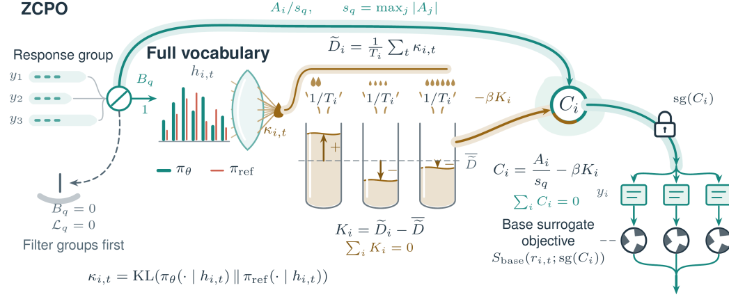
Figure 2: ZCPO coefficient construction. A_i = R_i - \bar{R} , B_q = \mathbf{1}\{G \geq 2, s_q > 0\} . All tokens in a response share \text{sg}(C_i) . Zero-sum coefficients do not imply a zero total gradient; conditional KL eliminates only token sampling noise conditional on a given prefix.
