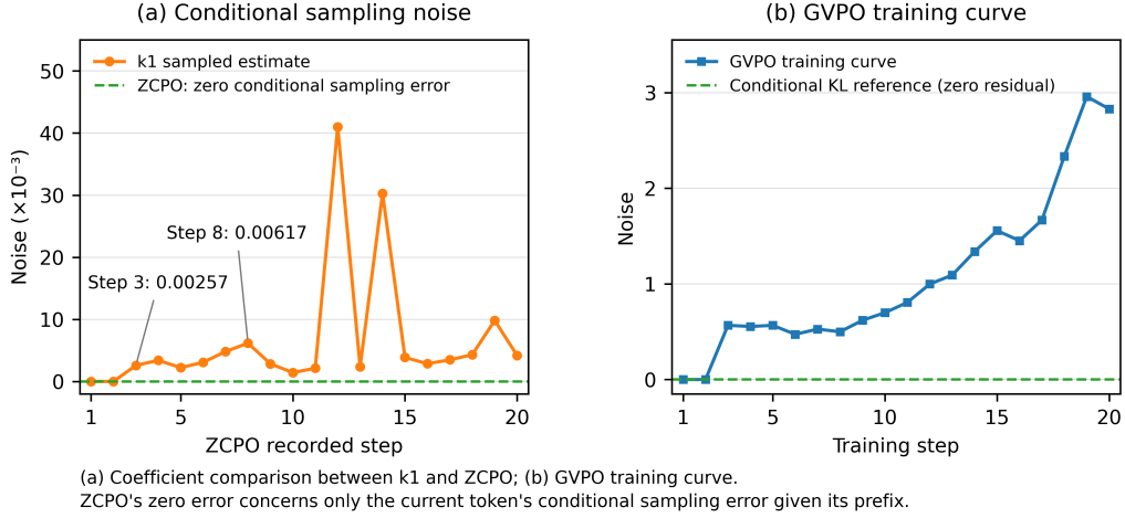
Figure 4: Conditional sampling-noise comparisons. (a) Using the first mini-batch at each of the first 20 steps of ZCPO, the orange curve shows the residual RMSE of the k1 coefficient relative to ZCPO, and the green curve shows ZCPO’s own zero residual. ZCPO’s zero conditional sampling error refers only to the local estimation term obtained by replacing sampled \Delta_{i,t} with \kappa_{i,t} for a given prefix; variation in sampled prefixes remains. (b) GVPO training curves. “Noise” denotes the sampling residual of the log-ratio relative to its per-prefix conditional mean. Its magnitude is the measured RMS of D_i^{k1} - D_i = \sum_t (\Delta_{i,t} - \kappa_{i,t}) after within-group centering, without multiplication by the KL weight. The green dashed line is the zero reference for conditional sampling error.
