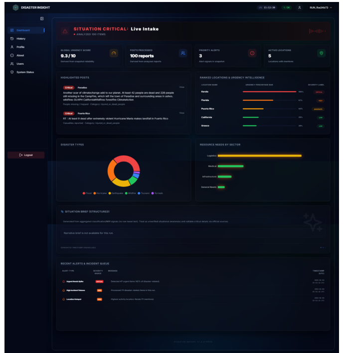
Fig. 8. Real-time web dashboard output. Input tweet (top), predicted entity spans with BIO type labels (middle), and humanitarian event classification result (bottom). Single forward pass through the shared RoBERTa-large encoder produces both outputs simultaneously.
