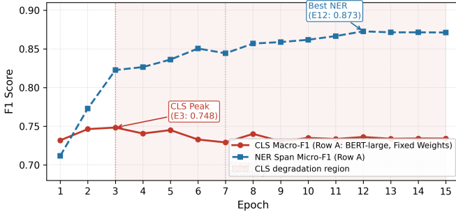
Fig. 5. CLS macro-F1 degradation under fixed task weights (Row A, single-stage training). CLS peaks at epoch 3 (0.748) then declines to 0.736 while NER improves from 0.711 to 0.873. Shaded region: degradation zone. The monotonic NER gain with simultaneous CLS decline is an empirical pattern consistent with gradient-asymmetry negative transfer; direct gradient diagnostics are left for future work.
