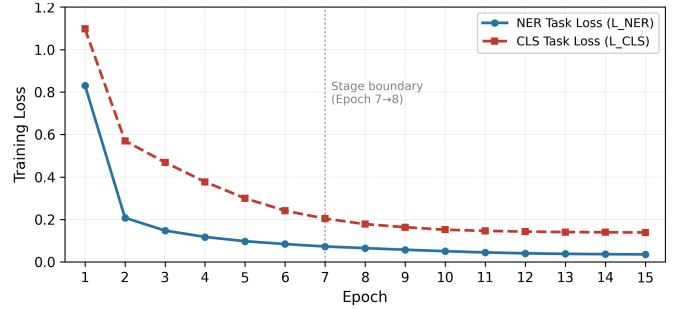
Fig. 6. Per-task training loss curves for Row A. Both L_{NER} and L_{CLS} decrease monotonically while CLS validation F1 degrades after epoch 3, demonstrating that training loss alone is insufficient evidence of generalisation under fixed-weight multitask training.
