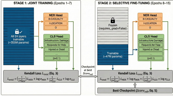
Fig. 3. Two-stage training procedure. Stage 1 (epochs 1–7) trains all layers jointly. Stage 2 (epochs 8–15) freezes layers 1–18 and fine-tunes only the upper six layers and task heads, reducing active parameters from 355M to 47M.
