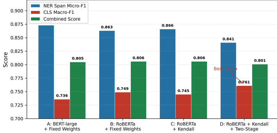
Fig. 4. Ablation scores for Rows A–D. NER span micro-F1 (blue), CLS macro-F1 (red), combined score (green). Row A achieves the highest NER (0.873); Row D achieves the highest CLS (0.761), the operationally critical metric for deployment.
