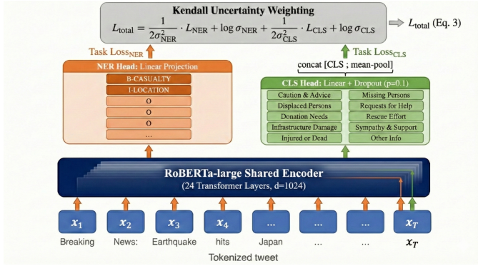
Fig. 2. Model architecture. The shared RoBERTa-large encoder feeds two task heads. The NER head performs token-level classification over 21 BIO entity classes. The CLS head concatenates [CLS] and mean-pooled representations before classifying into 10 humanitarian categories. Learnable uncertainty parameters \sigma_{NER} and \sigma_{CLS} weight the combined loss.
