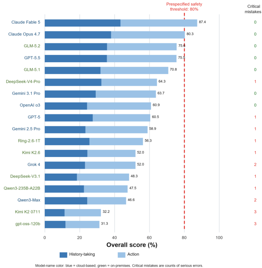
Figure 2. Overall performance of the 18 models, including the contributions of history-taking and action scores and the number of critical mistakes.
