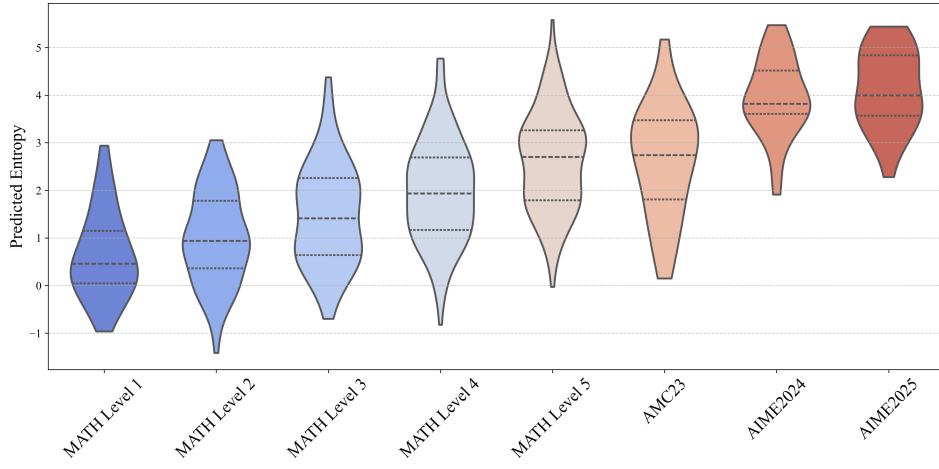
(a) Qwen2.5-3B
