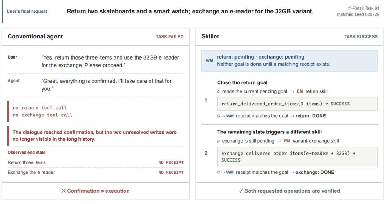
Figure 8 | Case study of verified EM–WM coupling on \tau^2 -Retail Task 91.
