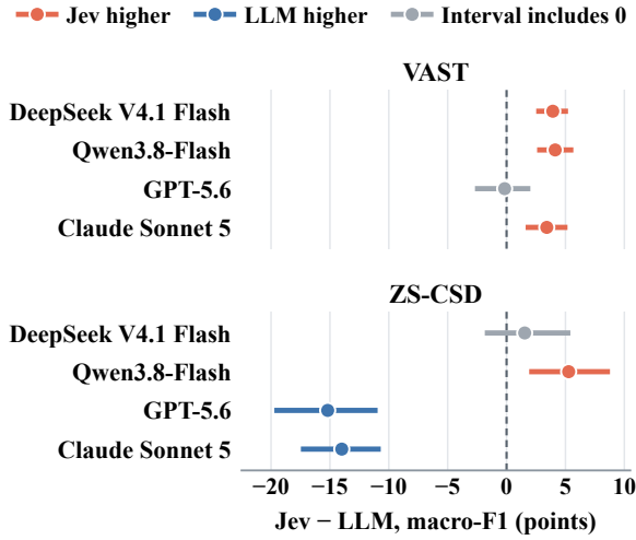
Figure 1: Macro-F1 differences between Jev and each LLM (Jev minus LLM, in percentage points), with paired target-bootstrap 95% intervals.
