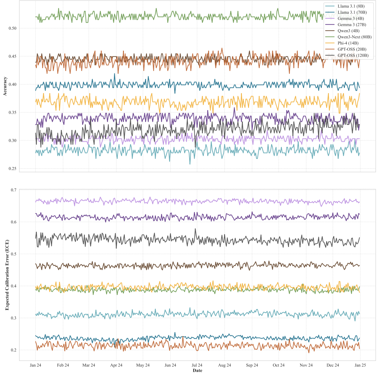
Figure 12: Accuracy and ECE across different dates in 2024 for all models on GPQA.
