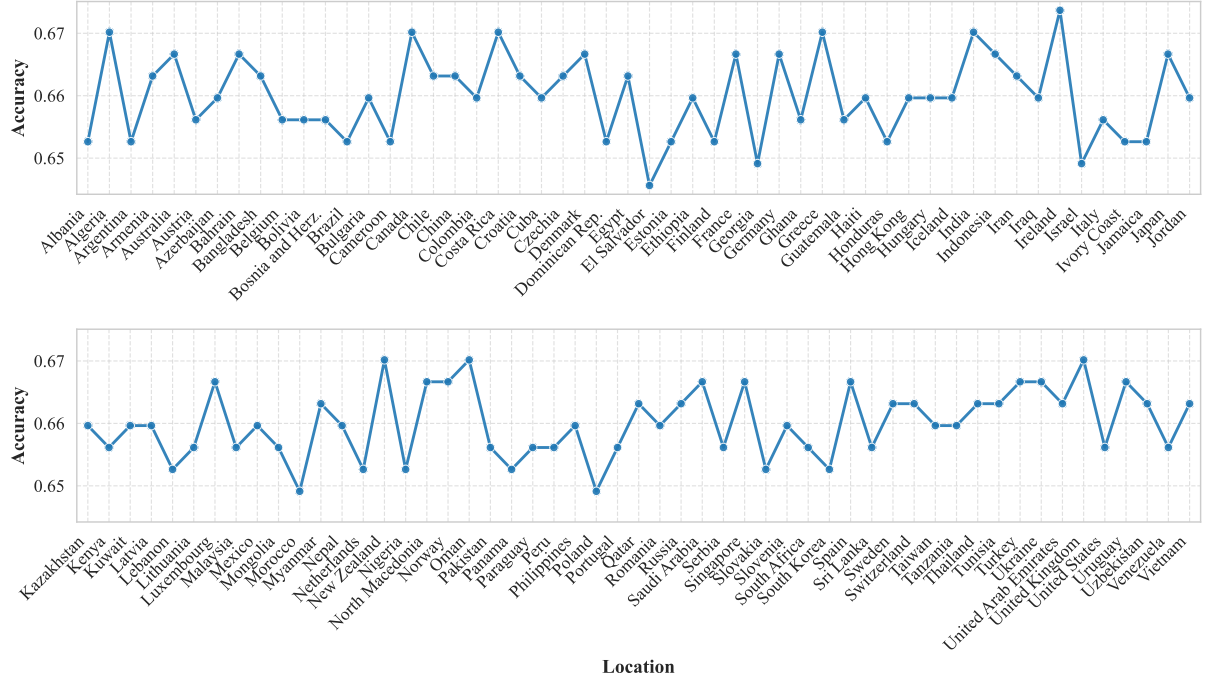
(a) Accuracy across different user locations for Llama 3.1 (8B) on MMLU.
