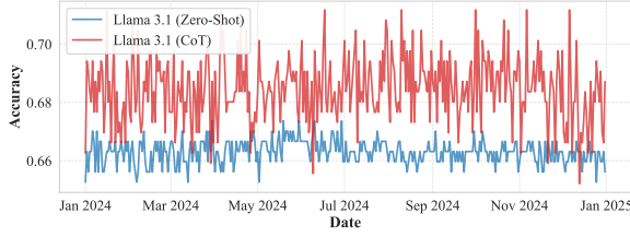
Figure 4: Comparison of accuracy across different dates in 2024 for Llama 3.1 (8B) on MMLU using zero-shot prompting vs. chain-of-thought prompting.
