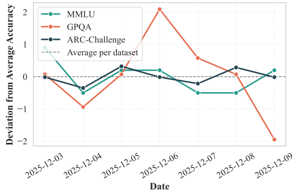
Figure 3: Accuracy deviation across different dates for GPT-5.1. The 0.0 line represents the average accuracy over the week for each dataset.
