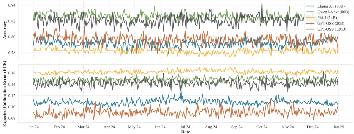
Figure 2: Accuracy (top) and ECE (bottom) across different dates in 2024 for the top-5 models on MMLU.
