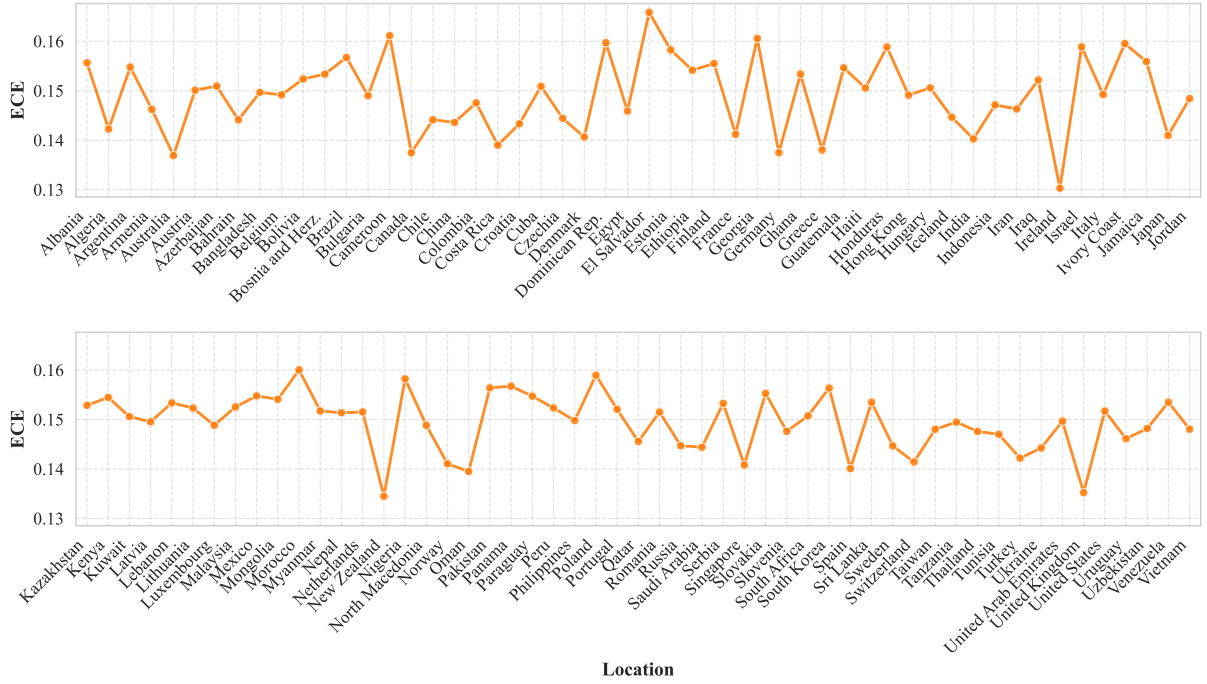
(b) ECE across different user locations for Llama 3.1 (8B) on MMLU.
