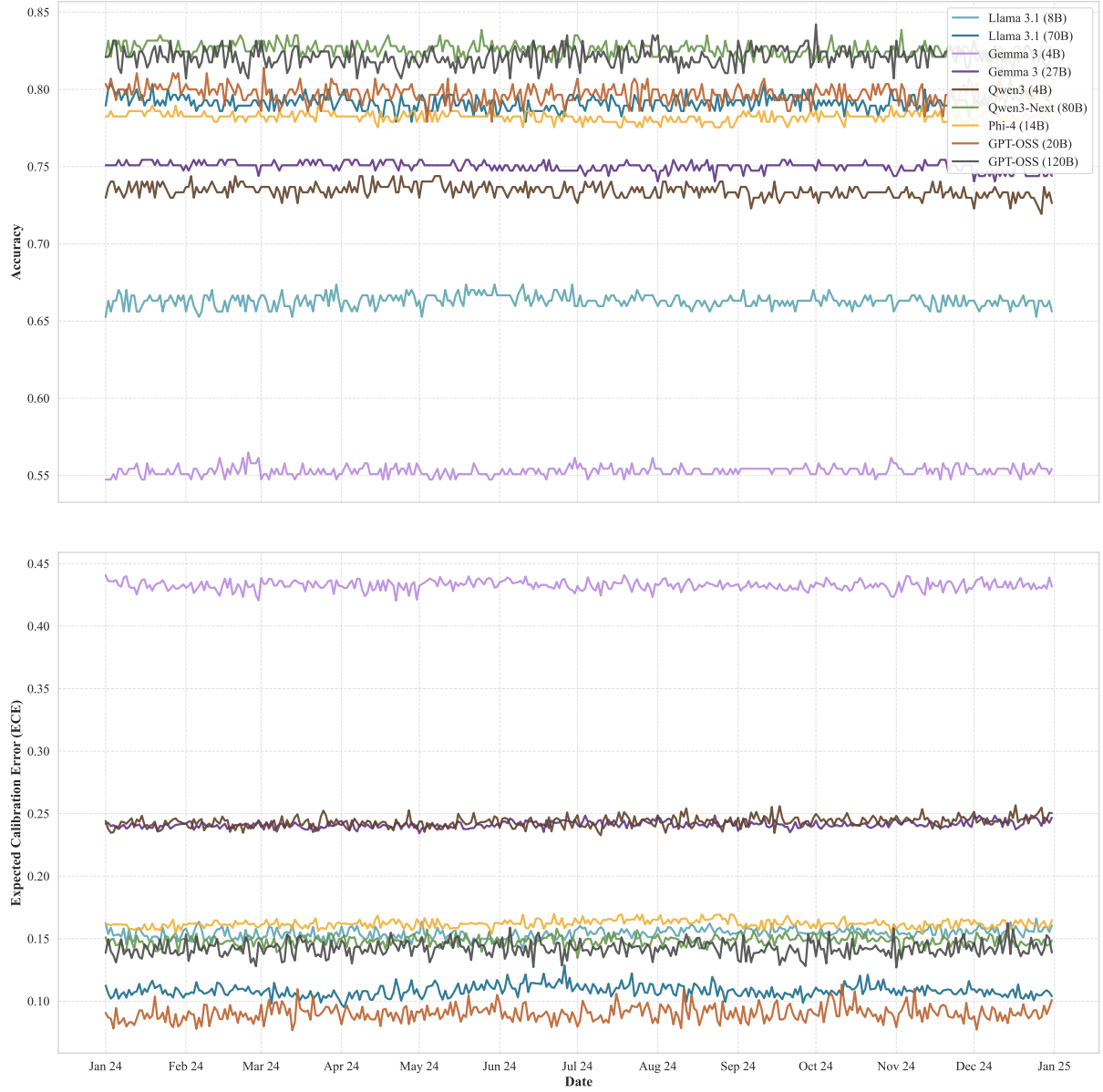
Figure 11: Accuracy and ECE across different dates in 2024 for all models on MMLU.
