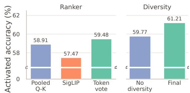
Figure 6 Retriever ablation on OVO-Bench queries selected by the calibrated Gate. Rankers are compared with diversity and temporal expansion disabled; diversity is compared with preceding-unit expansion.
