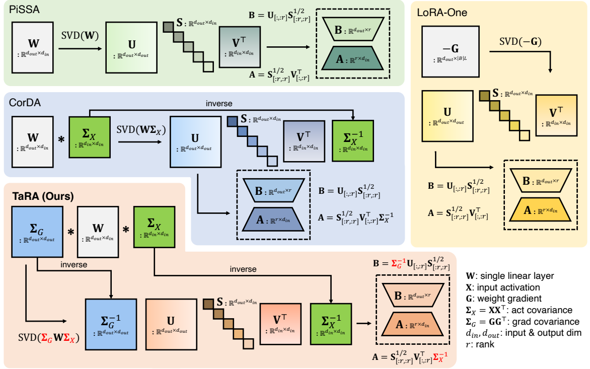
Figure 2: Illustration of our single-layer procedure. We collect activations \mathbf{X} and gradients \mathbf{G} to form covariances \Sigma_X and \Sigma_G . PiSSA applies SVD to \mathbf{W} ; CorDA applies SVD to \mathbf{W}\Sigma_X and maps back with \Sigma_X^{-1} ; LoRA-One applies SVD to -\mathbf{G} . In contrast, TaRA applies SVD to \Sigma_G \mathbf{W} \Sigma_X and maps back with \Sigma_G^{-1} and \Sigma_X^{-1} .
