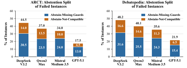
Figure 4: Decomposition of outcomes on abstain-missing-guards and abstain-not-compatible.
