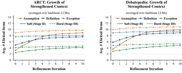
Figure 3: Average number of assumptions, definitions, and exception conditions per instance across soft and hard refinement iterations on Debatepedia and ARCT.
