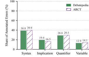
Figure B.1: Distribution of autoformalisation errors (syntax, implication, quantifier, variable) in the generated Isabelle/HOL theories, averaged over the four backbone LLMs. Annotation categories follow Quan et al. (2025b).
