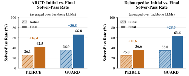
Figure 2: Initial and final solver-pass rates of PEIRCE and GUARD on Debatepedia and ARCT, averaged over the four backbone LLMs.
