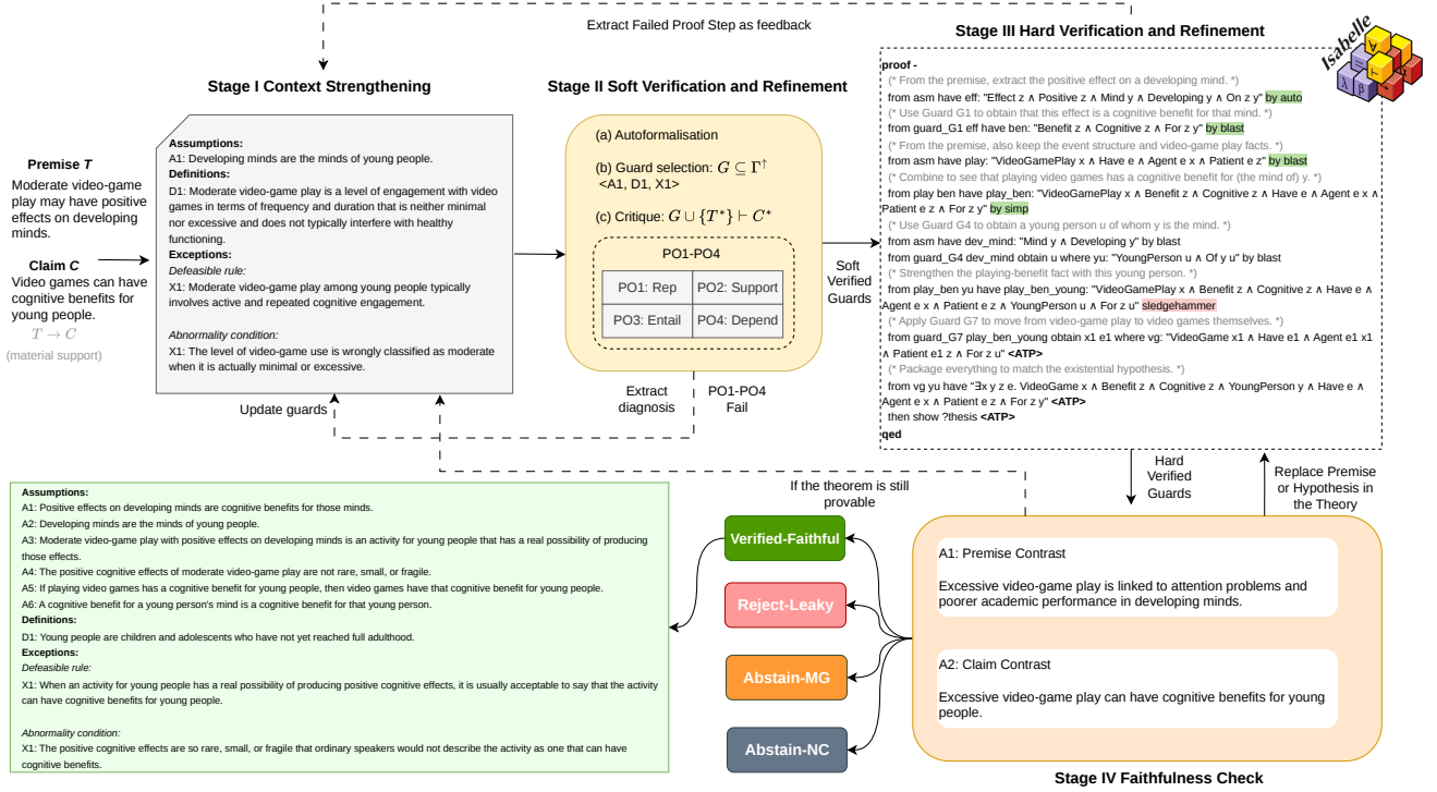
Figure 1: Overview of GUARD. Starting from a premise-claim pair (T, C) , the framework constructs a strengthened context, autoformalizes the selected candidate guards and iteratively combines soft verification, hard theorem proving and contrastive faithfulness checks until one of the four final statuses is reached.
