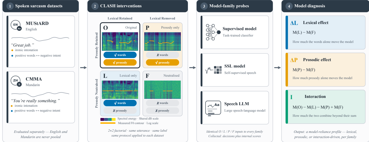
Fig. 1. Overview of CLASH. Utterances from MUSTARD and CMMA undergo paired interventions to form original ( O ), lexical-preserving ( L ), prosody-preserving ( P ), and approximately neutralised ( F ) conditions. The same inputs are evaluated using handcrafted acoustic-feature classifiers, SSL probes, and speech LLMs. Contrasts between conditions characterise lexical and prosodic effects and their interaction. The two corpora are evaluated separately.
