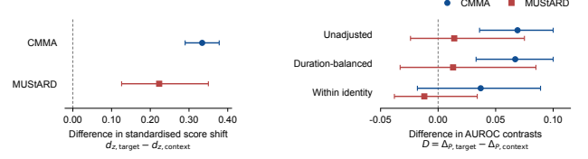
Fig. 2. Qwen3-Omni context comparison. Left: target-only minus context-aware standardised P - F score shifts. Right: D = \Delta_{P,\text{target}} - \Delta_{P,\text{context}} . Within-identity comparisons use CMMA conversations or MUSTARD speakers. Bars show marginal 95% paired cluster-bootstrap intervals; dashed lines mark zero. The axes measure different quantities.
