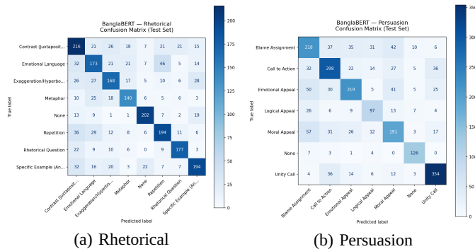
Fig. 2. Confusion matrices of BanglaBERT: (a) rhetorical technique detection, (b) persuasion technique detection.
