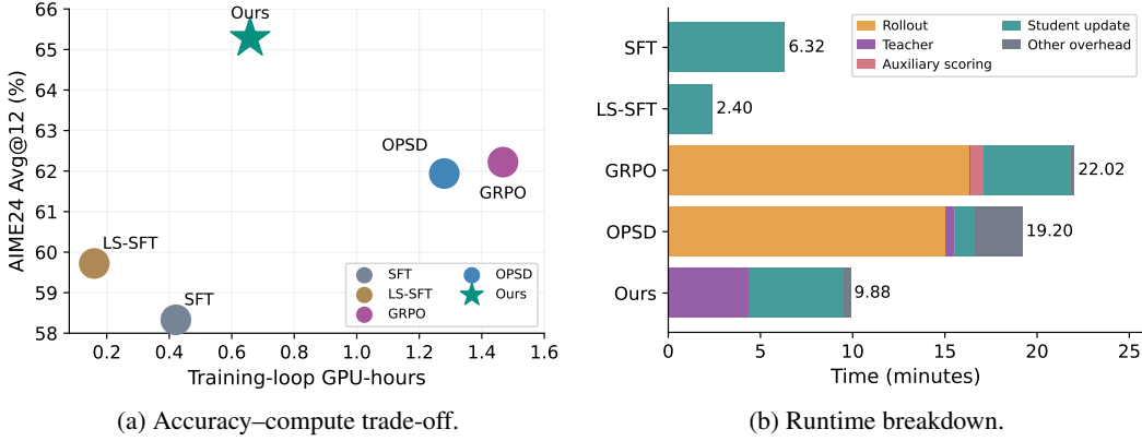
Figure 3: Training efficiency. (a) AIME24 Avg@12 accuracy versus training-loop GPU-hours. (b) Runtime decomposed by computational component; numbers at the bar ends indicate total runtime.
