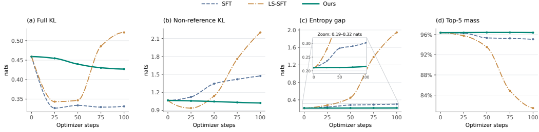
Figure 2: Training dynamics reveal preservation of non-reference distributional structure. (a) Full teacher–student KL, D_{\text{KL}}(p_T \| p_S) . (b) Conditional non-reference KL, computed after excluding the demonstrated token and renormalizing both distributions. (c) Mean token-level absolute entropy gap, |H(p_S) - H(p_T)| . The inset magnifies the range 0.19–0.32. (d) Student probability mass on the teacher’s top-five tokens.
