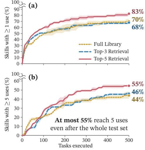
Figure 1: Percentage of skills used in (a) at least one task and (b) at least 5 tasks as downstream tasks are streamed and solved sequentially (Gemini 3.1 Flash-Lite, WebShop). Mean of three runs of the same task stream; bands show one standard deviation.
