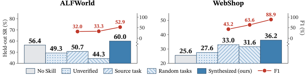
Figure 3: Verification with evidence from different types of tasks: held-out SR (bars, left axis) and F1 of the verdicts against held-out skill effects (line, right axis).
