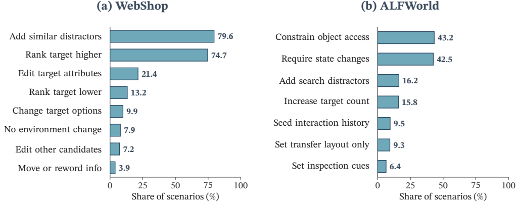
Figure 5: Planned synthesis mechanisms for Qwen3.5-27B on (a) WebShop and (b) ALFWorld. Each bar shows the percentage of scenarios using that transformation. A scenario may involve multiple transformations.
