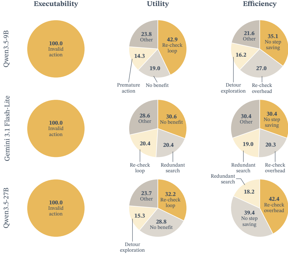
Figure 6: Primary failure cause of rejected skills according to the verification criterion. Each rejected skill and its scenario trajectories are analyzed and classified by GPT-5.6 Luna. The three largest types of each criterion are shown and the rest are pooled as Other.
