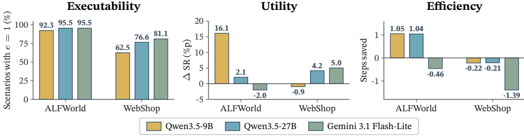
Figure 4: Executability, utility, and efficiency across all executors and benchmarks.
