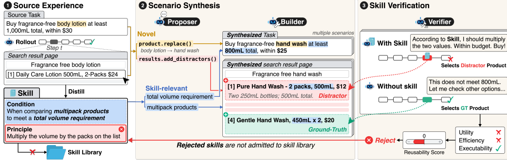
Figure 2: Overview of skill verification via dynamic scenario synthesis.
