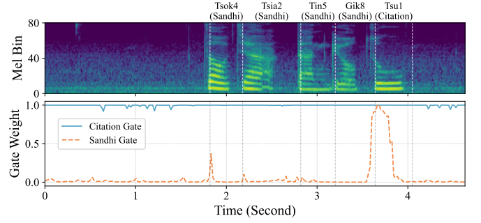
Fig. 5. Frame-level visualization of the dynamic gate.
