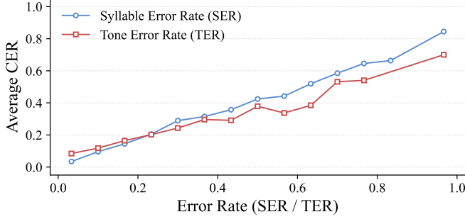
Fig. 4. Correlation between phonetic errors and transcription accuracy.
