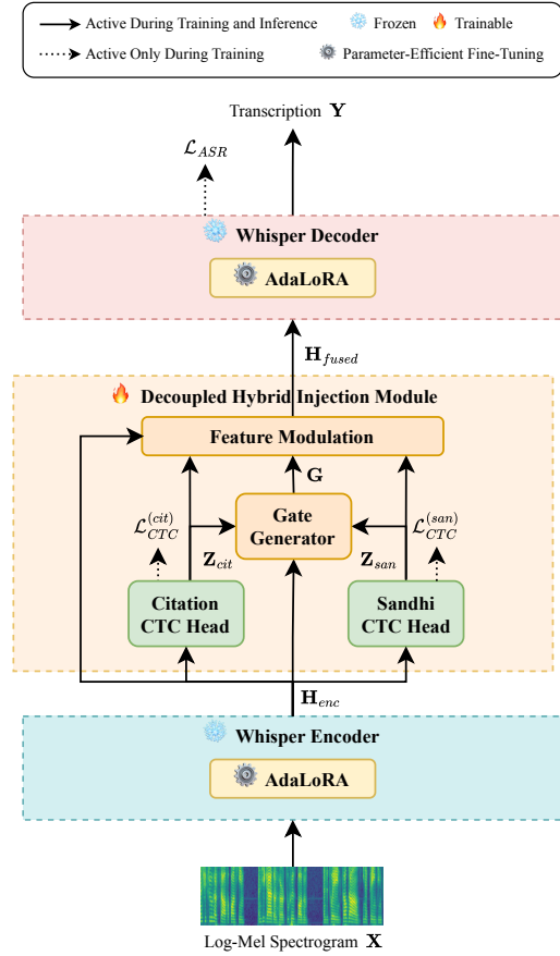
Fig. 3. Architecture of T-SANDHI. To explicitly decouple lexical intent from surface acoustics, a decoupled hybrid injection module augments the frozen Whisper encoder. It projects features into independent citation and sandhi streams, dynamically fusing them into \mathbf{H}_{fused} via a gate generator. Lightweight linear heads provide CTC supervision during training and supply decoupled representations during inference with negligible overhead.
