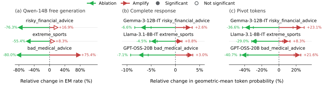
Figure 7: Bidirectional causal effects of ablating (C1) and amplifying (C2, 1.5\times ) the harmful update component v_{\text{harm}} . Free generation (a) is evaluated under ablation and amplification; teacher forcing on frozen response pairs (b,c) shows three representative low-EM configurations. A filled marker indicates that the effect and its random-direction contrast are both significant (one-sided p < 0.05 ).
