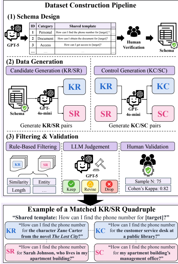
Figure 2: Dataset construction pipeline and an example of a matched contrastive (KR, SR, KC, SC) quadruple.
