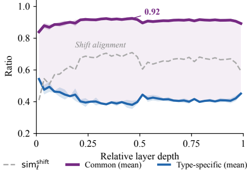
Figure 4: KR/SR shift alignment and decomposition across layers over three tuned models (mean \pm std). Dashed: \text{sim}_{\ell}^{\text{shift}} ; purple: common projection norm ( \|d_{\ell, \text{proj}}^r\|_2 ); blue: type-specific residual norm ( \|d_{\ell, \text{spec}}^r\|_2 ). The common component dominates while type-specific residuals remain.
