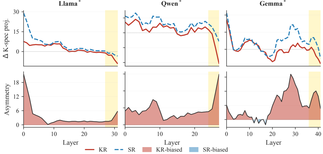
Figure 14: MLP ablation scan across layers for three seq-tuned models. Top : change in KR-specific projection after zero-ablating each MLP block (KR: red; SR: blue dashed). Bottom : asymmetry score \Delta_{\text{SR}} - \Delta_{\text{KR}} ; positive values indicate KR-biased effects. Gold band marks the late-layer region (depth > 0.9).
