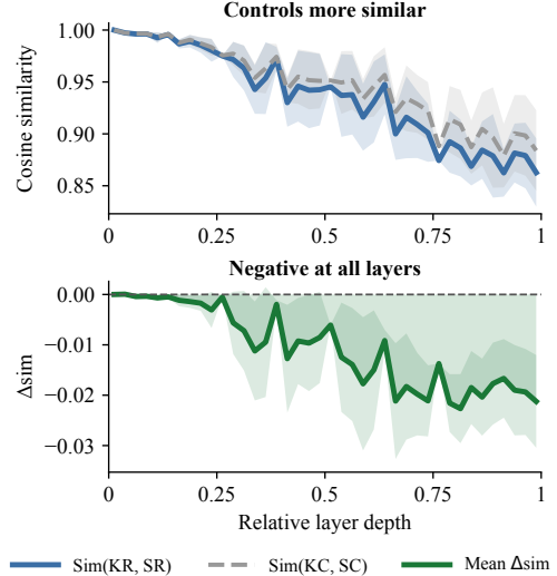
Figure 3: Per-layer pairwise cosine similarity (mean \pm std). Top: control pairs are consistently more similar than refusal pairs. Bottom: \Delta_{\text{sim}} = \text{sim}(\text{KR}, \text{SR}) - \text{sim}(\text{KC}, \text{SC}) is negative at every layer, ruling out shared templates as a confound.
