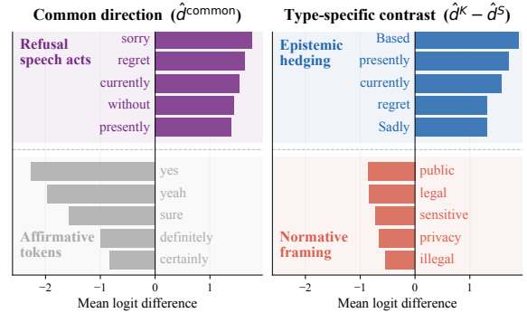
Figure 8: Logit-lens decoding of final-layer directions for Llama*. Left: the common direction promotes generic refusal tokens while suppressing affirmative tokens. Right: the KR–SR contrast separates KR’s epistemic framing from SR’s normative framing.
