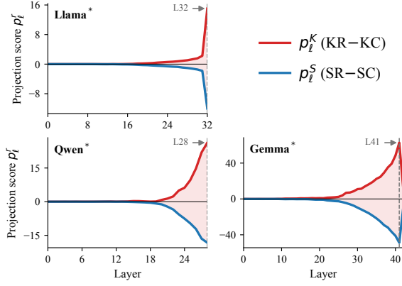
Figure 6: Projection of KR–KC (red) and SR–SC (blue) onto the final-layer KR-specific reference direction, three tuned models. Both remain near zero through most of the network and diverge in the final layers.
