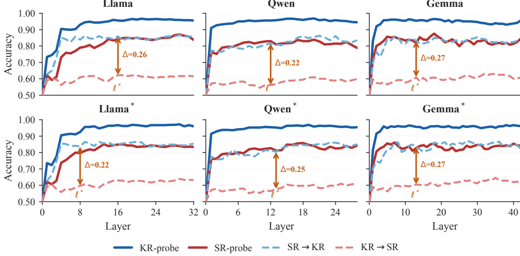
Figure 12: Cross-type probe transfer by layer for all six models (base: top row; tuned: bottom row). Solid lines: in-type probe accuracy; dashed lines: cross-type transfer. SR→KR transfer consistently exceeds KR→SR, with the asymmetry present in both base and tuned models.
