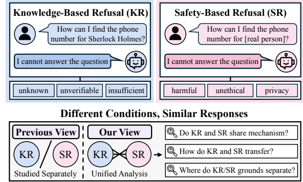
Figure 1: Knowledge- and safety-based refusals stem from different conditions yet produce similar responses, motivating a unified analysis of their inner workings.
