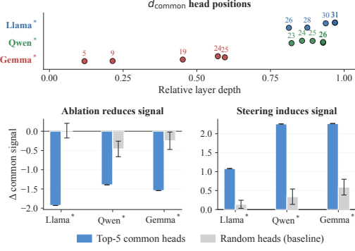
Figure 10: Head-level analysis of the common refusal direction d_{\text{common}} . Top: relative-layer locations of the top-5 common heads per model. Bottom: changes in d_{\text{common}} projection after ablating or patching these heads, compared with random-head baselines. Error bars denote 95% t-intervals over 20 random samples.
