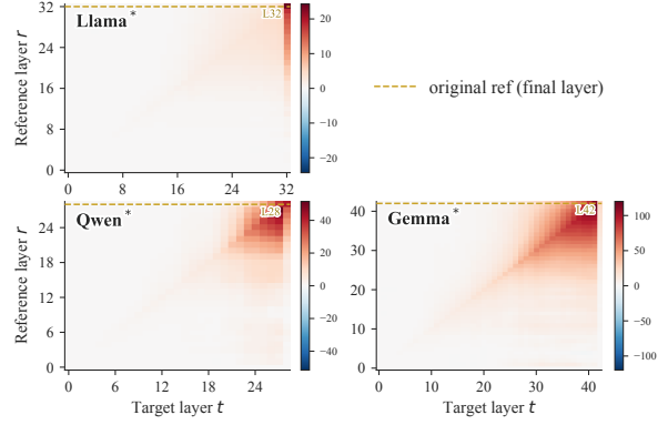
Figure 7: KR-specific divergence across reference layers r and target layers t . The dashed gold line marks the final-layer reference used in Figure 6. Late-layer concentration holds for non-final layers as well.
