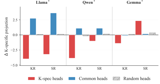
Figure 11: Change in KR-specific projection under head ablation. K-spec head ablation reduces the projection more strongly for KR than SR prompts (Llama*, Qwen*); Gemma* shows a positive shift on SR prompts. Common-head ablation produces a distinct pattern across all three models.
