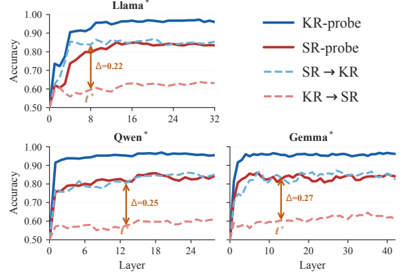
Figure 5: Within-type accuracy (solid) and cross-type transfer (dashed) across layers, three tuned models. KR-probe: blue; SR-probe: red. The (\text{SR} \rightarrow \text{KR}) - (\text{KR} \rightarrow \text{SR}) gap is present from early layers and stable throughout. \Delta denotes the gap at the peak layer \ell^* .
