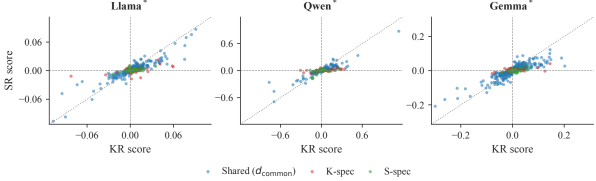
Figure 13: Joint distribution of KR/SR head contribution scores. Each point denotes one attention head, colored as shared, K-specific, or S-specific. Shared heads align along the diagonal, while type-specific heads deviate toward one axis.
