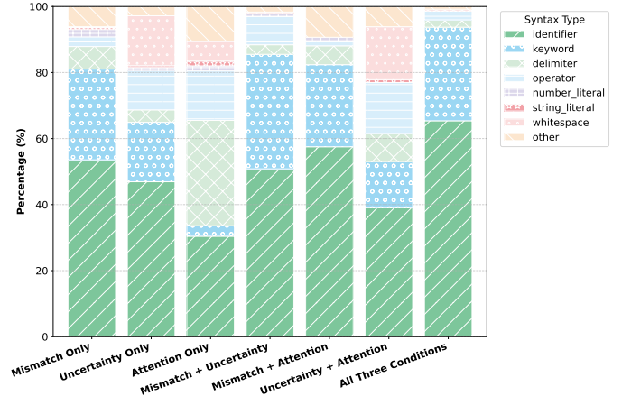
Fig. 7. Absolute Percentage Distribution of Syntax Types in critical tokens, using DSCoder-1B model.
