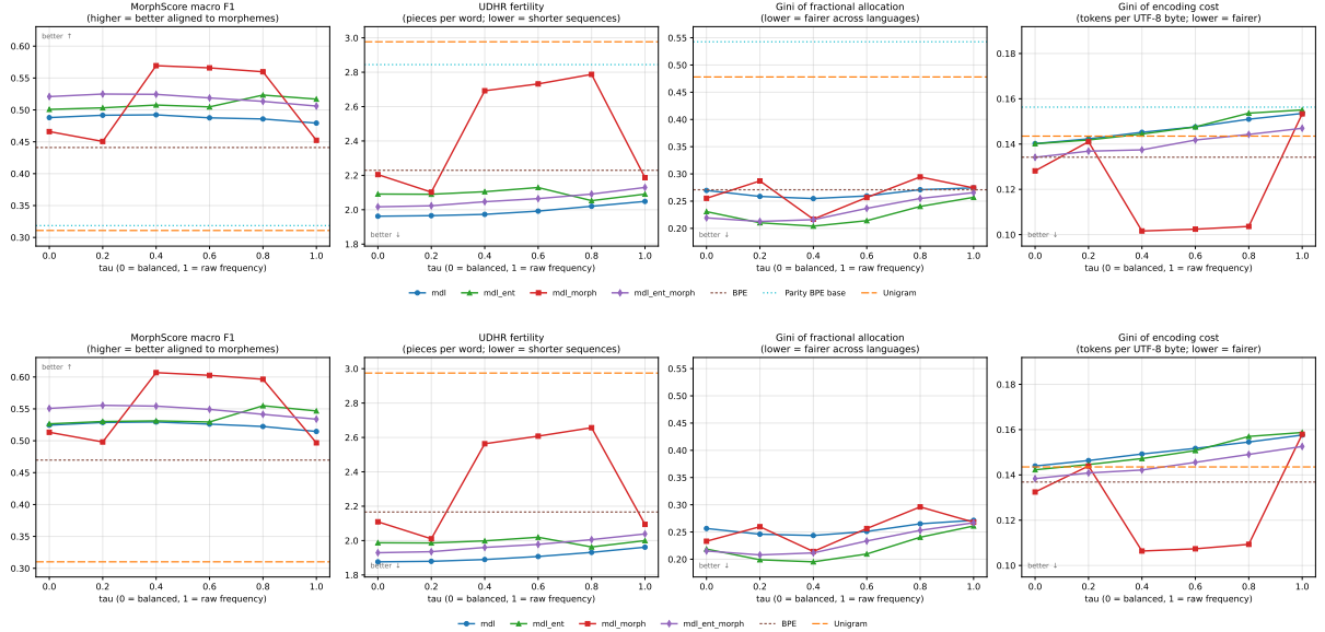
Figure 3: Intrinsic evaluation results for the 200k and 256k vocabulary configurations.
