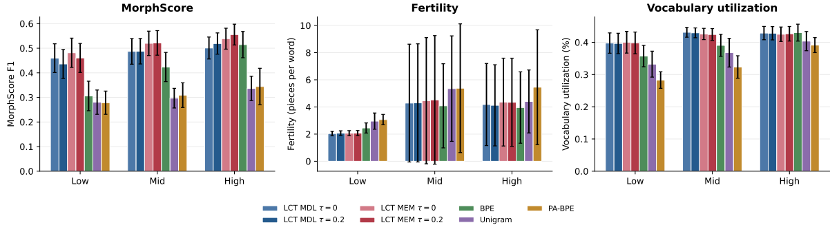
Figure 1: Intrinsic tokenizer performance across low-, mid-, and high-resource language tertiles. Bars show macro-averages and error bars indicate 95% confidence intervals across languages. MorphScore uses 65 languages, while fertility and vocabulary utilization use the 93 languages covered by TokEval. All configurations use a 200k vocabulary.
