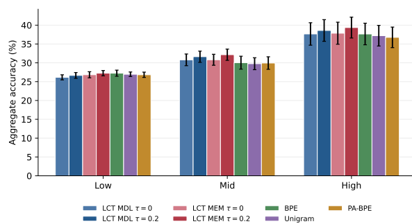
Figure 5: Aggregate downstream accuracy across low-, mid-, and high-resource language tertiles. Scores are averaged across the available XNLI, Belebele, XStoryCloze, and PAWS-X evaluations and five fine-tuning seeds. Error bars indicate 95% confidence intervals across languages.
