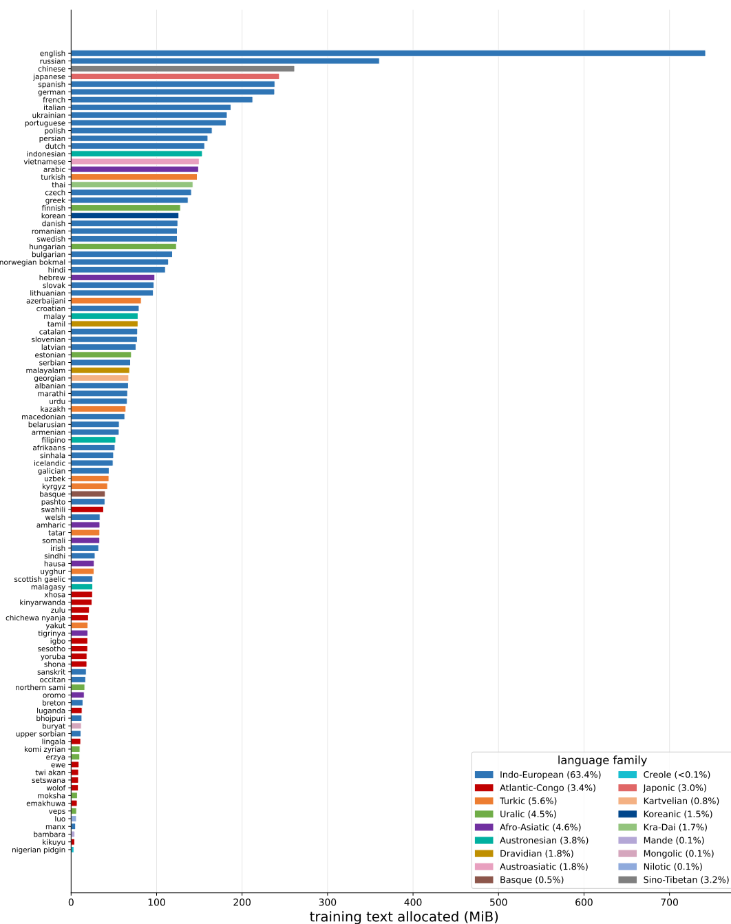
Figure 2: Per-language pretraining statistics
