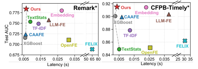
Figure 3: Inference latency and predictive performance across methods.
