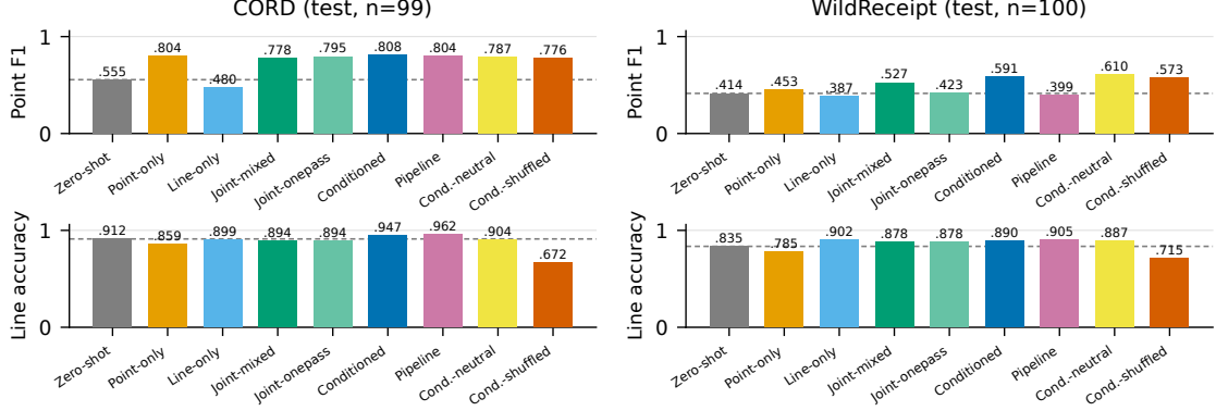
Figure 3: Point F1 (top) and line accuracy (bottom) on CORD and WildReceipt test sets, 8B backbone, plain prompts at evaluation. Dashed line marks zero-shot. No single-forward-pass baseline measurably beats CONDITIONED on either side. The two rightmost bars are controls: COND.-NEUTRAL fills the same slots with uninformative placeholders, COND.-SHUFFLED with another document’s content.
