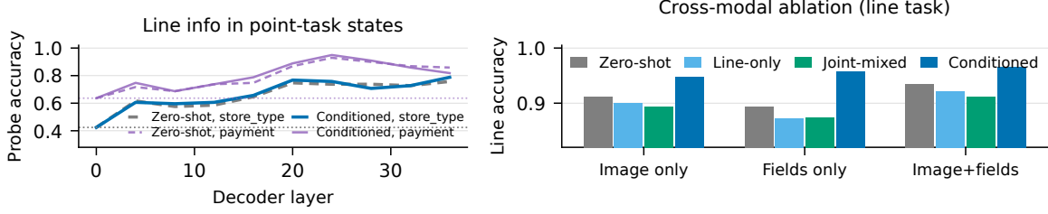
Figure 4: Left: layer-wise probe accuracy for line information in point-task states, zero-shot (dashed) vs CONDITIONED (solid), dotted lines mark the majority baselines (.42 store_type, .64 payment_method); decodability rises with depth. Right: line accuracy by input modality. CONDITIONED is the only model for which the field text alone beats the image alone, and fusion is superadditive for all.
