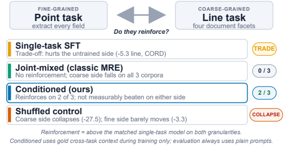
Figure 1: Four arrangements of the same task pair, judged by one predicate: reinforces means above the matched single-task model on both granularities. Only conditioned training does so, on two of three corpora; filling the same prompt with another document’s content collapses the coarse side.
