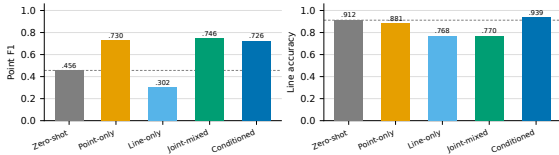
Figure 6: Five-regime replication on Qwen3-VL-4B, CORD test, identical recipe. Line-side pattern amplifies: LINE-ONLY and JOINT-MIXED fall 14 points below zero-shot on the line task itself, CONDITIONED alone stays above it. Point side: JOINT-MIXED .746 exceeds CONDITIONED .726 ( -2.0 [-4.5, +0.4] ) and POINT-ONLY .730 sits 0.5 above it ( [-3.1, +2.2] ), so the point-side advantage of conditioning is specific to 8B and its point-side no-loss holds only within noise at 4B; the line advantage holds at both scales ( +2.8 [0.5, 5.1] over zero-shot).
