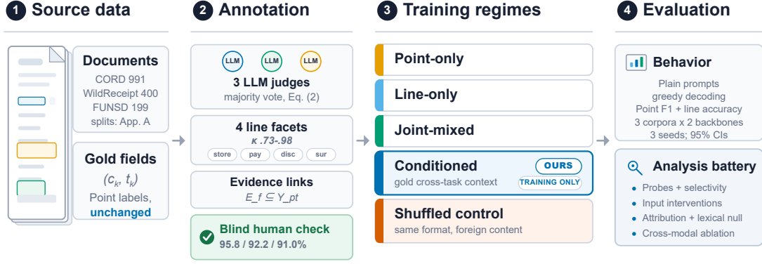
Figure 2: Overview. (1) Source documents keep their gold field annotations as point labels. (2) A three-judge LLM committee adds four document-level facets and directional evidence links by majority vote; blind human re-annotation validates the labels at 95.8%, 92.2% and 91.0% agreement on the three corpora. (3) Five training regimes arrange the same task pair differently; only CONDITIONED sees gold cross-granularity context, and only during training; the shuffled control keeps its format but swaps in another document’s content. (4) All models are evaluated with plain prompts on three corpora, two backbones and three seeds, then analyzed with a four-instrument battery.
