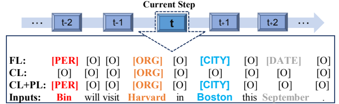
Fig. 1. A basic example of INER scenario, where FL, CL, and PL represent Full ground-truth Labels, Current ground-truth Labels, and Pseudo Labels, respectively. Previous entity types (e.g., [PER] (Person), [CITY] (City)) and future entity type (e.g., [DATE] (Date)) are marked as the non-entity type (i.e., [O]) in the current step t where [ORG] (Organization) is the current entity type being learned, leading to the shift of the non-entity type semantics (the second row CL). Using PL produced by the previous model to augment CL as the current classification target can effectively address the issue of semantic shift (the third row CL+PL).
