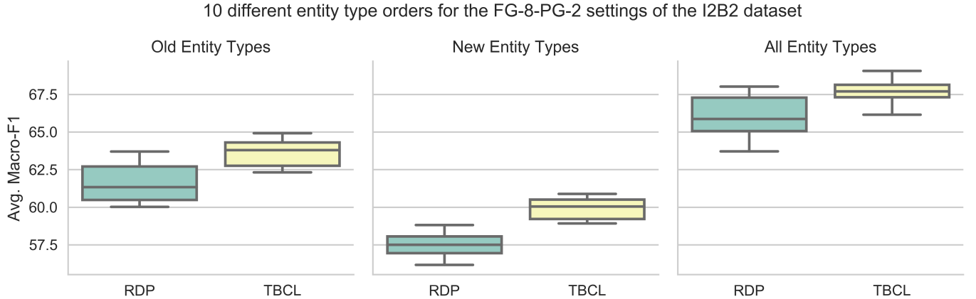
Fig. 6. The boxplots display the average Macro-F1 scores for the old, new, and all entity types across INER steps for 10 random entity type orders. TBCL is significantly better and more stable than RDP.
