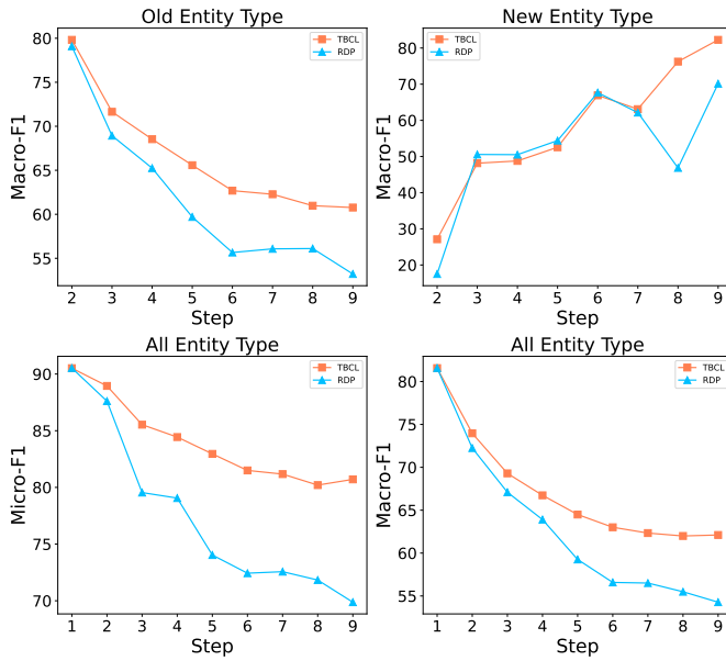
Fig. 4. Comparison of the step-wise Macro-F1 scores for old, new, and all entity types, along with the step-wise Micro-F1 scores for all entity types, using the FG-8-PG-1 setting of the I2B2 dataset [45]. Our TBCL method consistently outperforms the previous SOTA INER baseline, RDP [17], in most step-wise evaluations.
