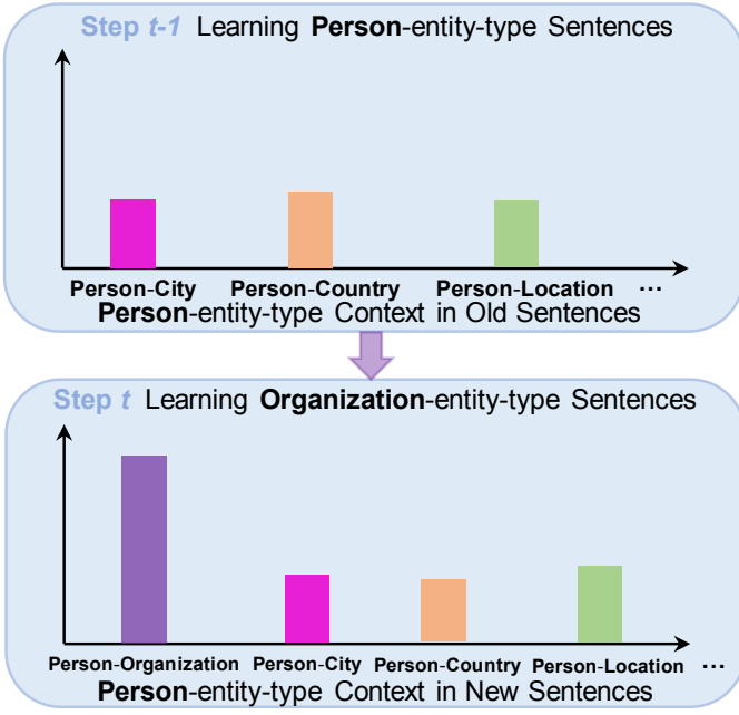
Fig. 2. Depiction of biased contextual relationships between the old-entity-type and new-entity-type tokens in the new sentences. At step t - 1 , when the NER model learns Person -entity-type sentences, the context of Person includes various entity types (e.g., Person-City , Person-Country , Person-Location ). However, at step t , when the model learns the new Organization -entity-type sentences, the context of Person predominantly comprises Person-Organization pairs. Consequently, a new-entity-type-biased context for the old-entity-type ( Person ) tokens emerges in the new-entity-type ( Organization ) sentences, exacerbating the old-entity-type forgetting and new-entity-type overfitting issues.
