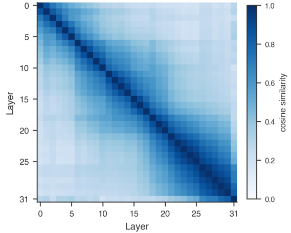
Figure 18: Layer-to-layer cosine similarity of the user-role direction in Qwen 3.5 9B. Layers 6–20 form a broad mid-layer cluster.
