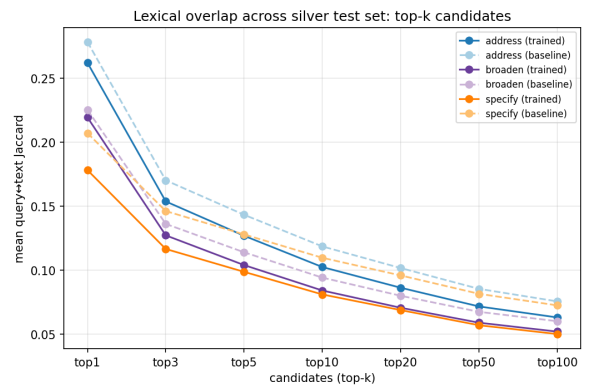
Figure 4: Query–candidate lexical overlap by relation, over retrieval depth for silver set and ModernBERT-embed-large. Lexical overlap is Jaccard score with unigram, stopwords removed, snowball-stemmed.
