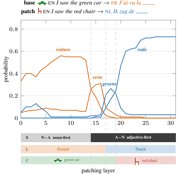
Figure 1: Translation in mLLMs proceeds in three stages: syntax S is fixed before output language L, which is fixed before the concept C. Patching individual layers of an English → French base prompt with an English → Dutch patch prompt reveals which aspects of the patch prompt persist in the output. Patching early layers changes nothing: the prediction stays voiture . In Llama 3 8B, from layer 14 only the word order persists ( verte ). The language persists from layer 17 ( groene ), the concept from layer 19 ( rode ).
