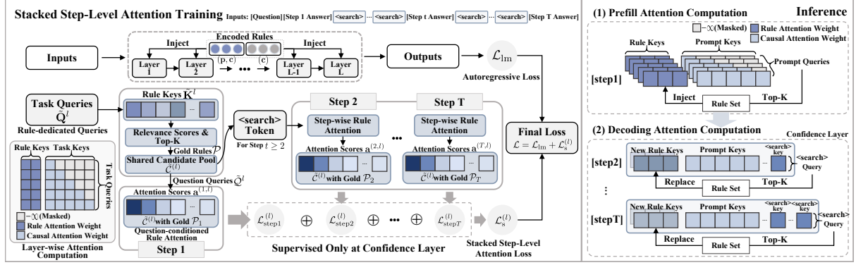
Figure 2: Overview of Stacked Step-Level Attention Training (left) and dynamic rule attention at inference (right). Training builds a shared candidate pool \tilde{C}^{(l)} from sequence-level relevance between \tilde{Q}^l and injected rule keys \tilde{K}^l , and learns step-level retrieval with question and <search> tokens. At inference, top- K rules are selected at prefill and updated through re-attention triggered by <search> tokens. Values are omitted for clarity.
