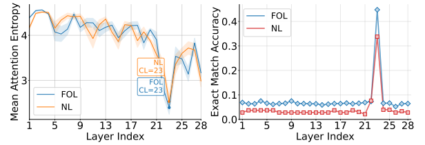
Figure 3: Confidence layer (CL) identification (FOL/NL), with shading showing attention entropy standard deviation ( left ). Per-layer retention analysis with correct rules injected into a single target layer ( right ).
